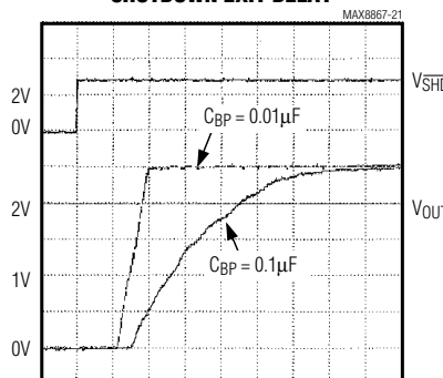
MAX886 E_K25 SHUTDOWN EXIT DELAY
