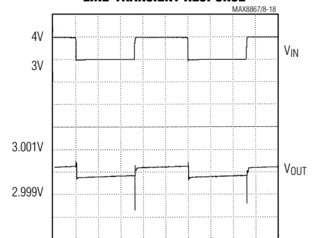
LINE-TRANSIENT RESPONSE
