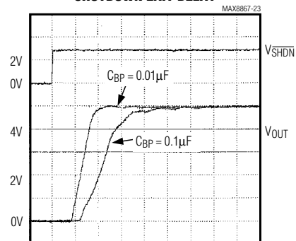
MAX886 E_K50 SHUTDOWN EXIT DELAY
