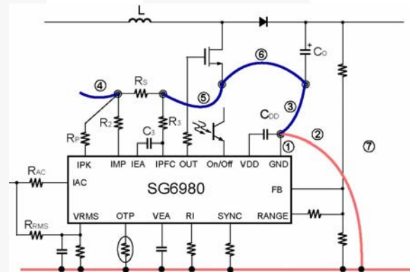
FIG. 7 PCB Layout
