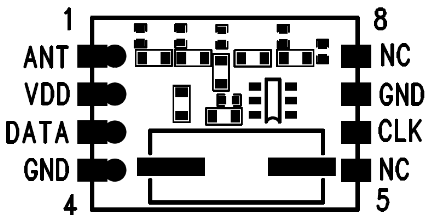
Figure 2. Pin Diagram
