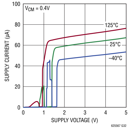
Supply Current vs Supply Voltage per Channel, -40°C, 25°C, 125°C
