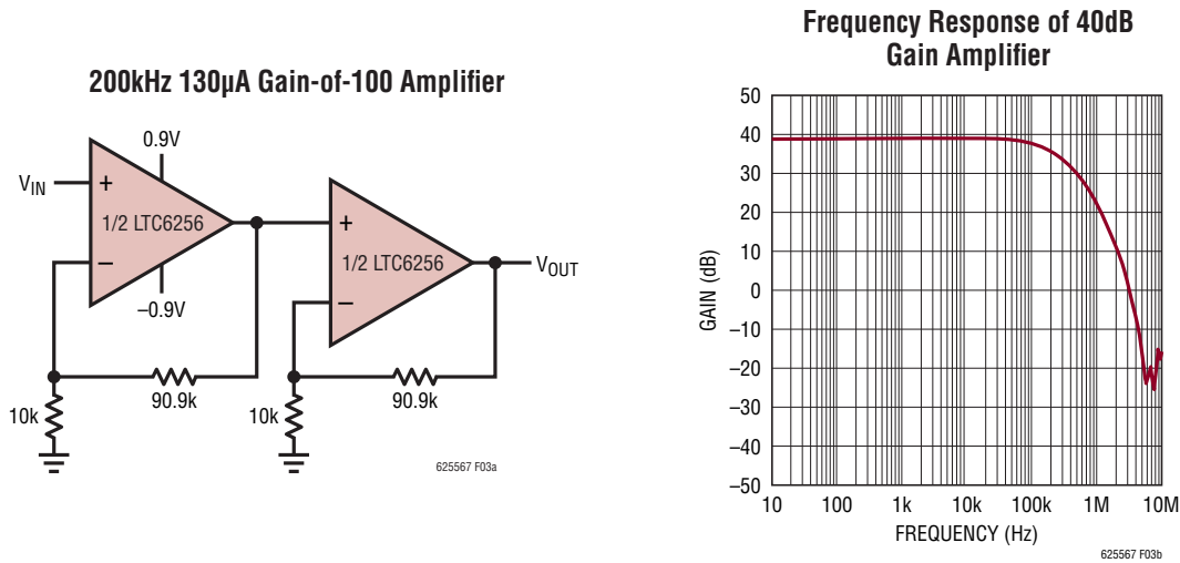
Figure 3. Gain of 100 Amplifier (3dB Bandwidth of 200kHz on 130μA Supply Current)
