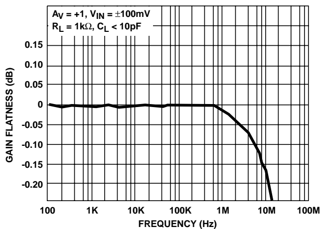
FIGURE 24. GAIN FLATNESS
