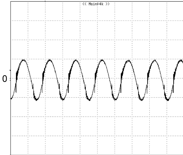
Figure 11: Input Terminal Ripple Current, i_c , at full rated output current and nominal input voltage with 12\mu\text{H} source impedance and 33\mu\text{F} electrolytic capacitor (500 mA/div, 2 us/div)
