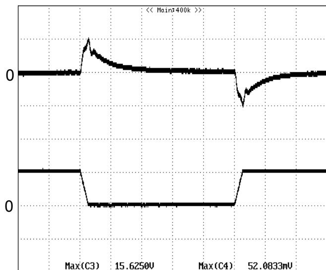
Figure 8: Output voltage response to step-change in load current (75%-50%-75% of I_{o, max} ; di/dt = 0.1A/\mu s ). Load cap: 10 \mu F tantalum capacitor and 1 \mu F ceramic capacitor. Top Trace: V_{out} (50mV/div, 200us/div), Bottom Trace: I_{out} (5A/div). Scope measurement should be made using a BNC cable (length shorter than 20 inches). Position the load between 51 mm to 76 mm (2 inches to 3 inches) from the module
