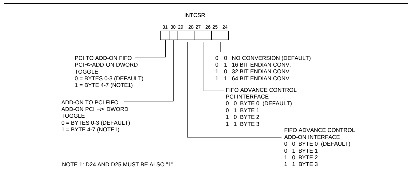
Figure 72. INTCSR FIFO Advance and Endian Control Bits
