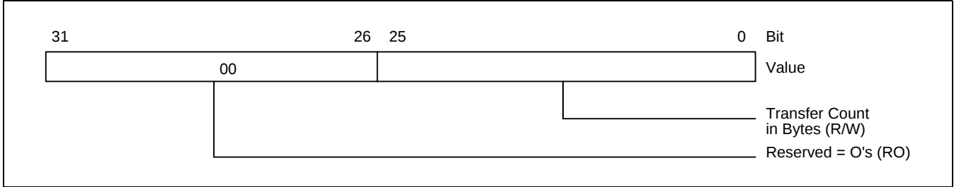
Figure 25. PCI Controlled Bus Master Write Transfer Count Register
