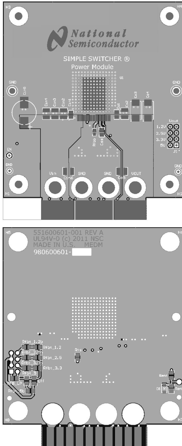
Figure 58. Layout example
