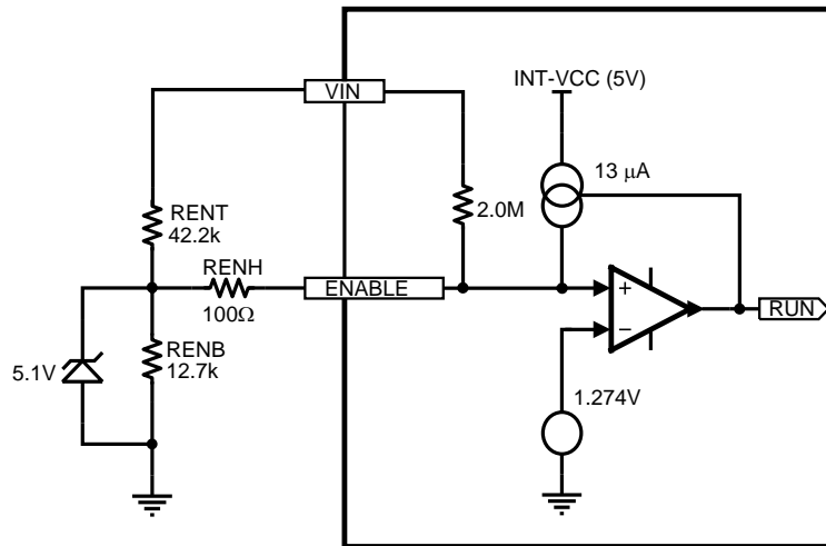
Figure 49. Enable input detail
