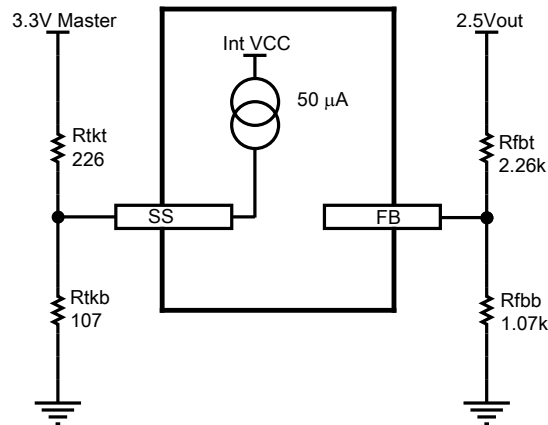
Figure 50. Tracking option input detail
