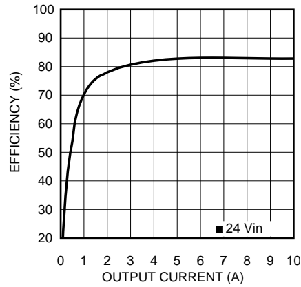
Figure 2. Efficiency V_{IN} = 24V V_{OUT} = 3.3V
