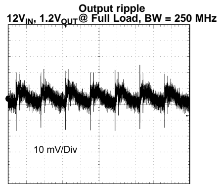
TIME (2 \mu s /Div) Figure 42.
