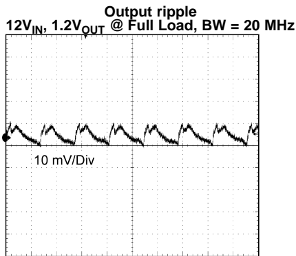
TIME (2 \mu s /Div) Figure 41.
