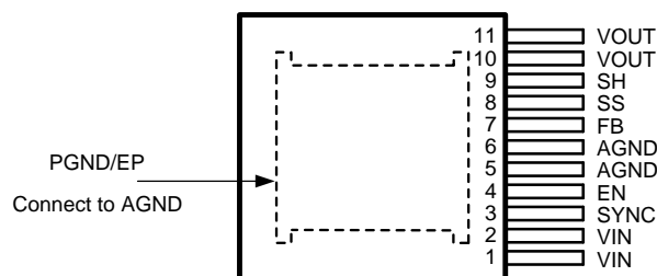
Figure 4. Top View 11-Lead PFM
