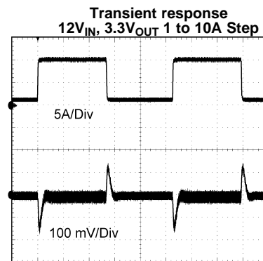
TIME (500 \mu s /Div) Figure 44.
