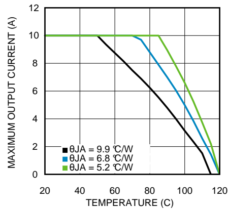
Figure 3. Thermal derating curve V_{IN} = 24V , V_{OUT} = 3.3V
