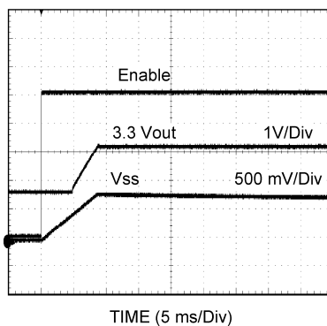
Figure 55. Pre-Biased Startup
