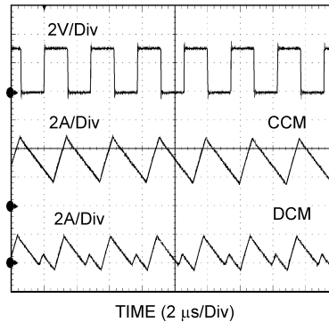
Figure 56. CCM and DCM Operating Modes V_{IN} = 12V , V_O = 3.3V , I_O = 3A/0.3A
