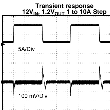
TIME (500 \mu s /Div)
