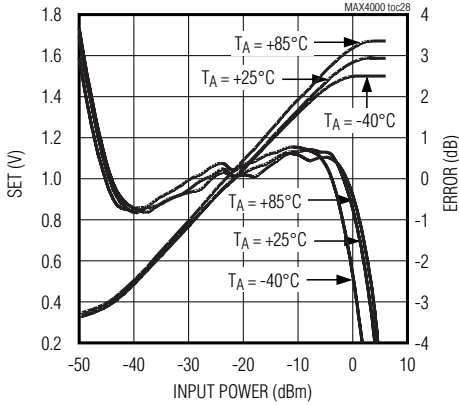
MAX4000 SET AND LOG CONFORMANCE vs. INPUT POWER AT 2.5GHz (uMAX)
