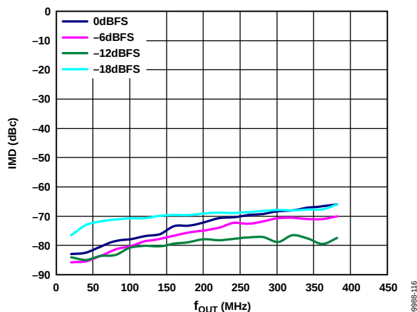
Figure 19. IMD vs. f_{OUT} over Digital Scale, 2x Interpolation, f_{DATA} = 400 MSPS, I_{FS} = 20 mA
