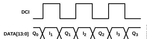
Figure 42. Timing Diagram for Word Mode
