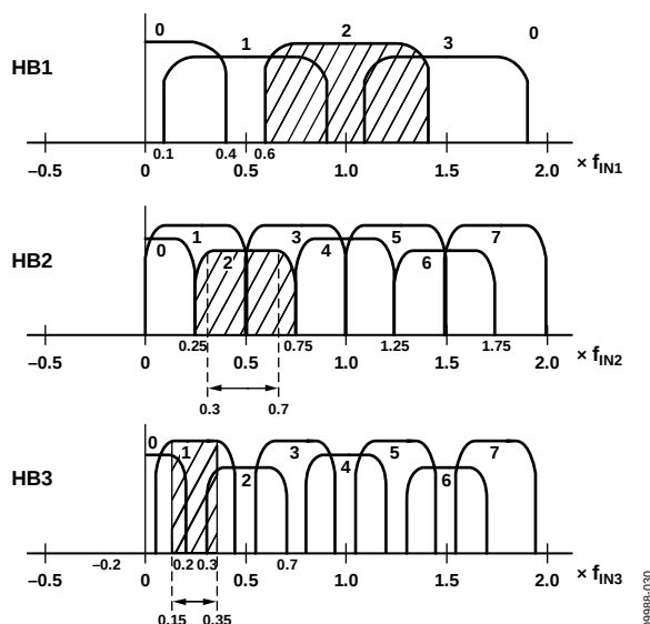
Figure 59. Signal Propagation for 8× Interpolation ( f_{\text{DATA}} Modulation)
