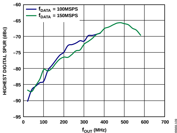
Figure 12. Highest Digital Spur vs. f_{OUT} over f_{DATA} , 8x Interpolation, Digital Scale = 0 dBFS, I_{FS} = 20 mA
