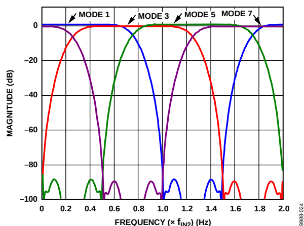
Figure 53. HB2, Odd Filter Modes
