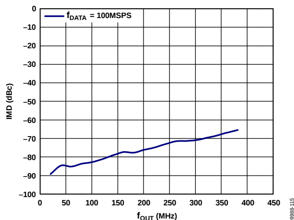
Figure 18. IMD vs. f_{OUT} 8x Interpolation, f_{DATA} = 100 MSPS, Digital Scale = 0 dBFS, I_{FS} = 20 mA
