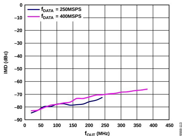
Figure 16. IMD vs. f_{OUT} over f_{DATA} 2x Interpolation, Digital Scale = 0 dBFS, I_{FS} = 20 mA
