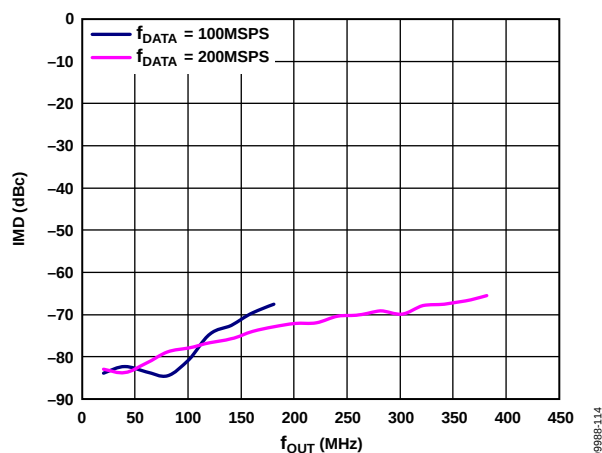
Figure 17. IMD vs. f_{OUT} over f_{DATA} 4x Interpolation, Digital Scale = 0 dBFS, I_{FS} = 20 mA
