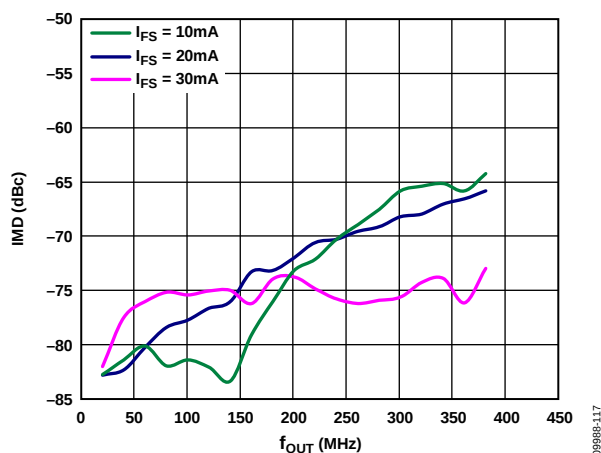
Figure 20. IMD vs. f_{OUT} over I_{FS} 2x Interpolation, f_{DATA} = 400 MSPS, Digital Scale = 0 dBFS
