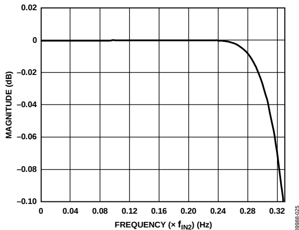
Figure 54. Pass-Band Detail of HB2
