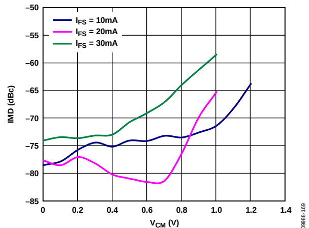
Figure 70. IMD vs. Output Common-Mode Voltage ( f_{OUT} = 161 MHz, R_{LOAD} = 50 \Omega Differential, I_{FS} = 10 mA, 20 mA, and 30 mA)
