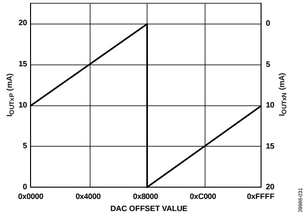
Figure 60. DAC Output Currents vs. DAC Offset Value
