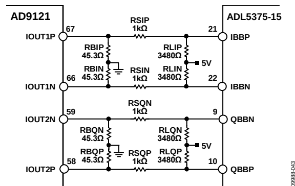
Figure 73. Passive, Level-Shifting Network for Biasing the ADL5375-15
