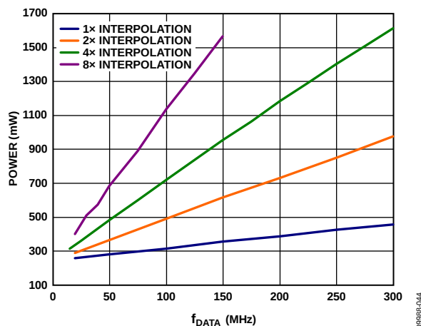
Figure 75. Total Power Dissipation vs. f_{\text{DATA}} Without PLL, Fine NCO, or Inverse Sinc
