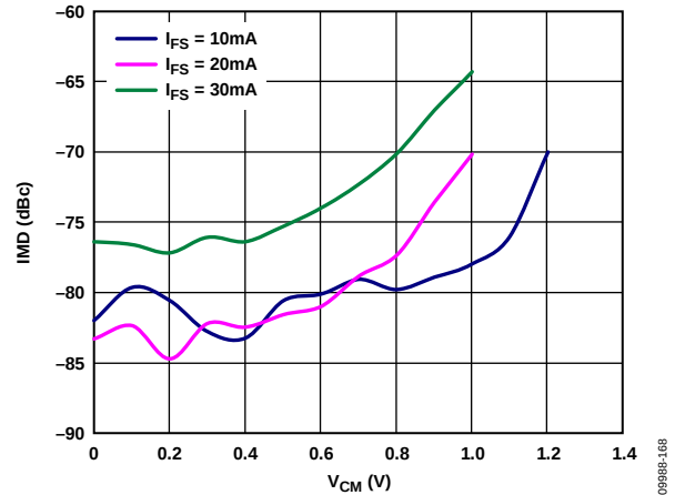
Figure 69. IMD vs. Output Common-Mode Voltage ( f_{OUT} = 61 MHz, R_{LOAD} = 50 \Omega Differential, I_{FS} = 10 mA, 20 mA, and 30 mA)
