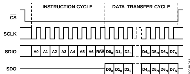
Figure 39. Serial Port Interface Timing, LSB First
