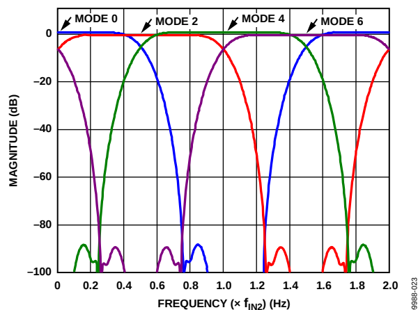
Figure 52. HB2, Even Filter Modes
