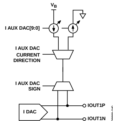
Figure 71. Auxiliary DAC Structure
