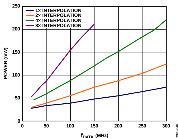
Figure 77. CVDD18 Power Dissipation vs. f_{\text{DATA}} with PLL Disabled
