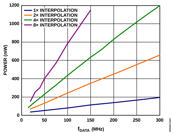
Figure 76. DVDD18 Power Dissipation vs. f_{\text{DATA}} Without Fine NCO or Inverse Sinc
