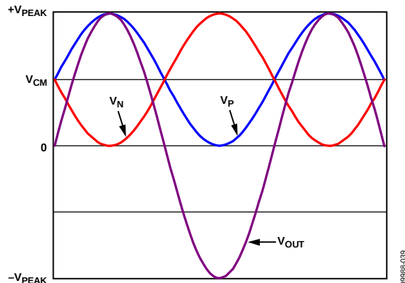
Figure 68. Output Voltage Waveforms
