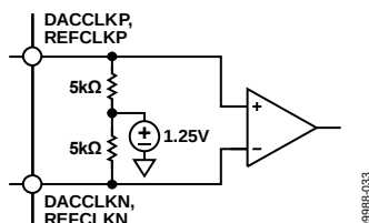
Figure 62. Clock Receiver Input Simplified Equivalent Circuit
