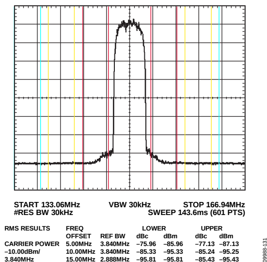
Figure 35. One-Carrier W-CDMA ACLR Performance, IF = ~150 MHz
