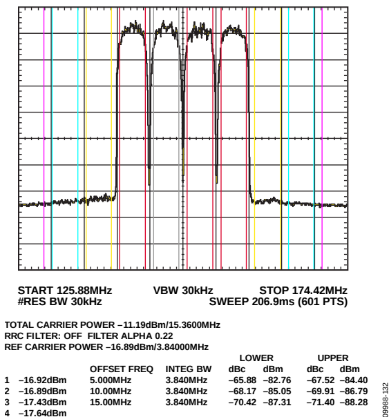
Figure 36. Four-Carrier W-CDMA ACLR Performance, IF = ~150 MHz
