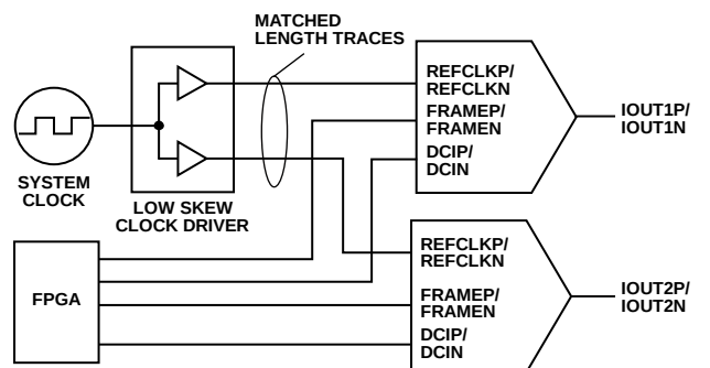
Figure 80. Typical Circuit Diagram for Synchronizing Devices
