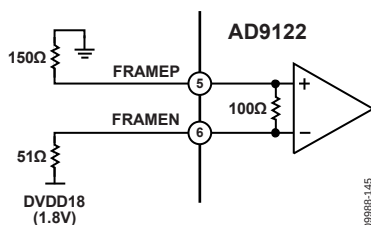
Figure 45. External Bias Circuit
