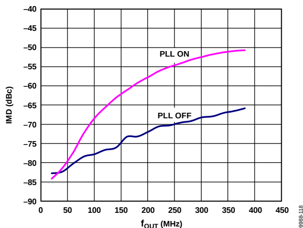
Figure 21. IMD vs. f_{OUT} 4x Interpolation, f_{DATA} = 200 MSPS, Digital Scale = 0 dBFS, I_{FS} = 20 mA, PLL On and PLL Off
