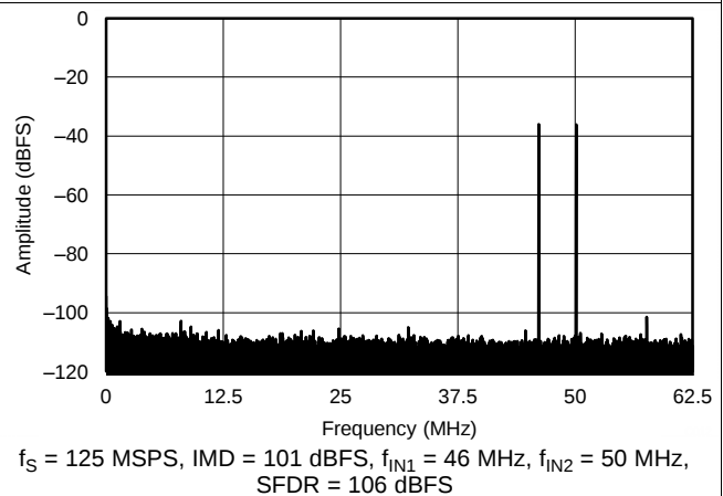
Figure 45. FFT for Two-Tone Input Signal ( -36\text{ dBFS} at 46 MHz and 50 MHz)
