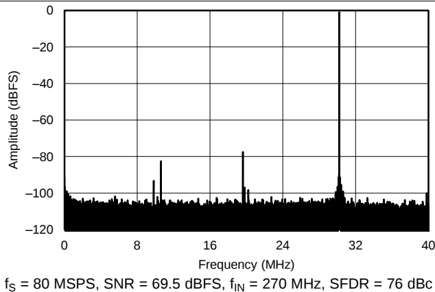
Figure 73. FFT for 270-MHz Input Signal, Dither On
