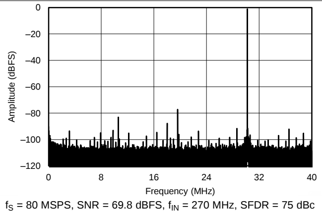
Figure 74. FFT for 270-MHz Input Signal, Dither Off
