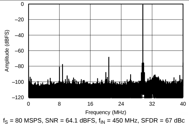
Figure 76. FFT for 450-MHz Input Signal, Dither Off
