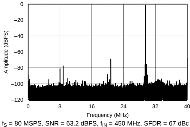
Figure 75. FFT for 450-MHz Input Signal, Dither On
