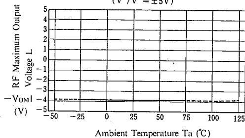
RF Maximum Output Voltage L vs. Temperature
