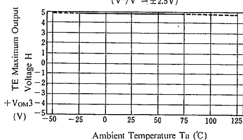
TE Maximum Output Voltage H vs. Temperature
