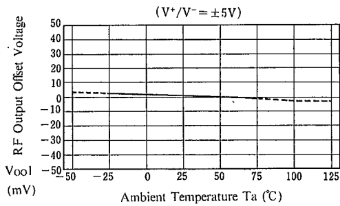
RF Output Offset Voltage vs. Temperature
