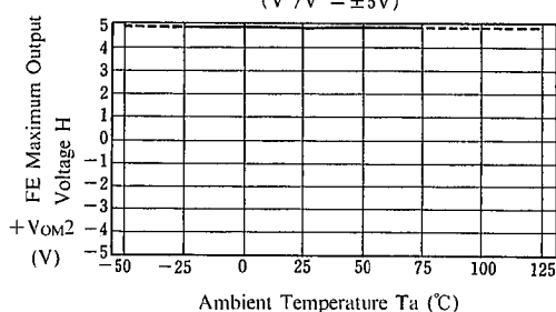
FE Maximum Output Voltage H vs. Temperature
