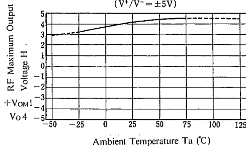
RF Maximum Output Voltage H vs. Temperature
