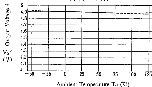
APC Vo4 vs. Temperature
