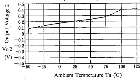
APC Vo2 vs. Temperature
