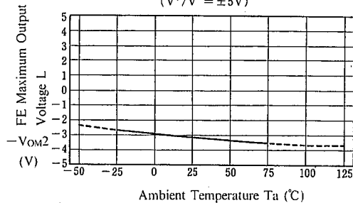
FE Maximum Output Voltage L vs. Temperature
