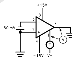
Test Circuit 2 (Emitter Output)
