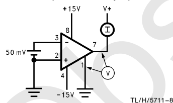
Test Circuit 1 (Collector Output)
