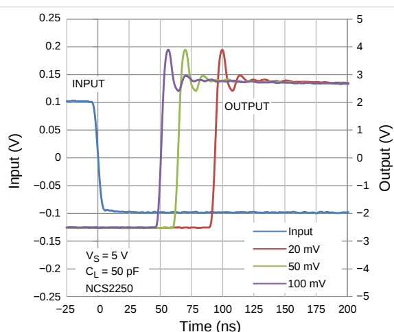
Figure 2. Transient Response at 5 V Supply with Varying Input Overdrive Voltages
