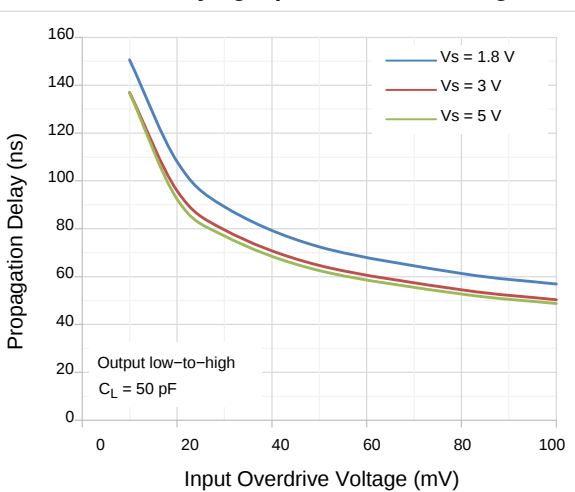
Figure 6. Output Low-to-High Propagation Delay vs. Input Overdrive Voltage
