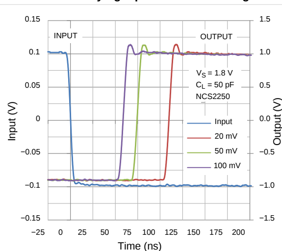
Figure 4. Transient Response at 1.8 V Supply with Varying Input Overdrive Voltages
