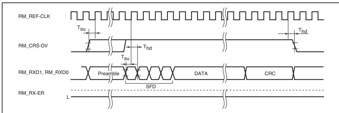
Figure 31.36 RMII Receive Timing (Normal Operation)
