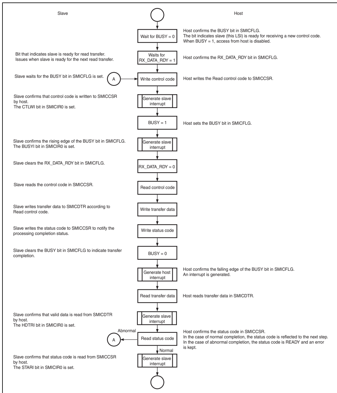
Figure 19.5 SMIC Read Transfer Flow
