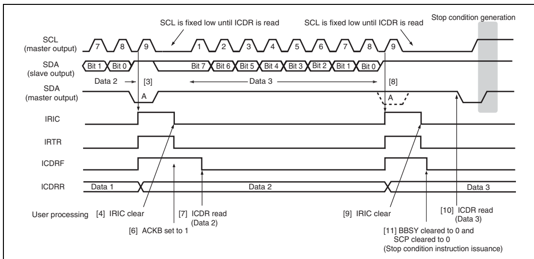
Figure 18.12 Stop Condition Issuance Timing Example in Master Receive Mode (MLS = WAIT = 0, HNDS = 1)
