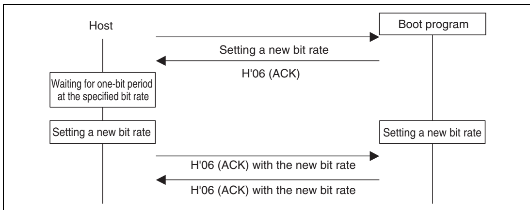
Figure 25.23 New Bit-Rate Selection Sequence
