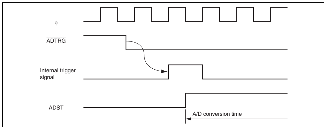
Figure 23.5 Timing of External Trigger Input
