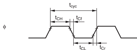
Figure 31.4 System Clock Timing
