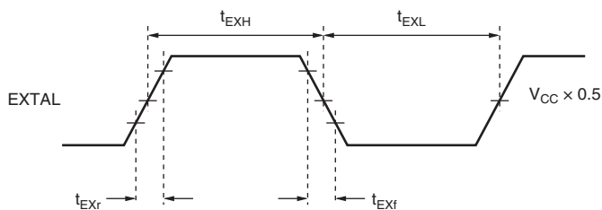
Figure 31.7 External Clock Input Timing
