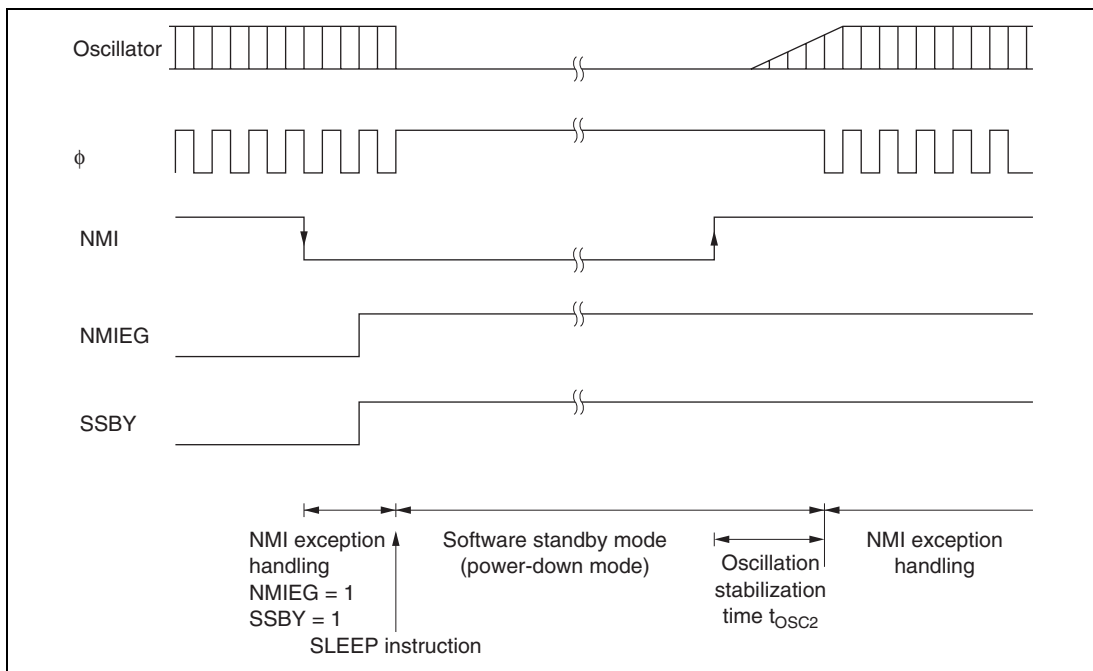
Figure 28.3 Software Standby Mode Application Example
