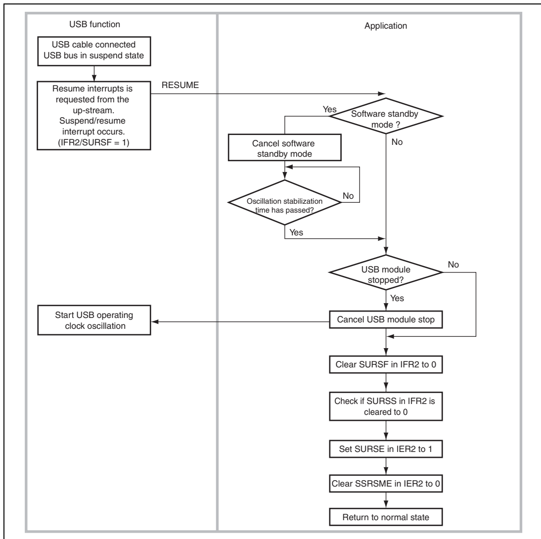
Figure 22.5 Resume Operation from Up-Stream
