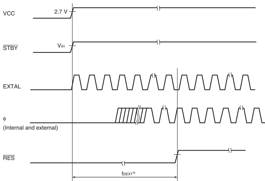
Figure 31.7 External Clock Input Timing
