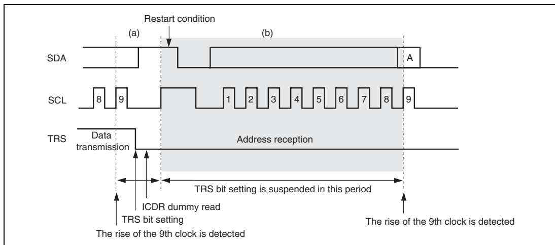
Figure 18.34 TRS Bit Set Timing in Slave Mode
