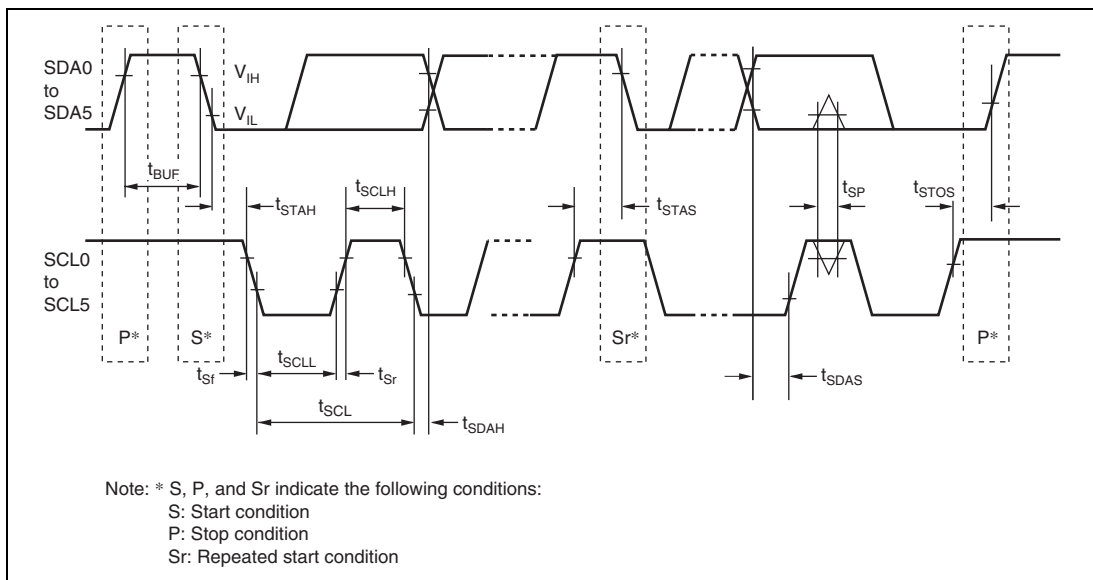
Figure 31.32 I²C Bus Interface Input/Output Timing
