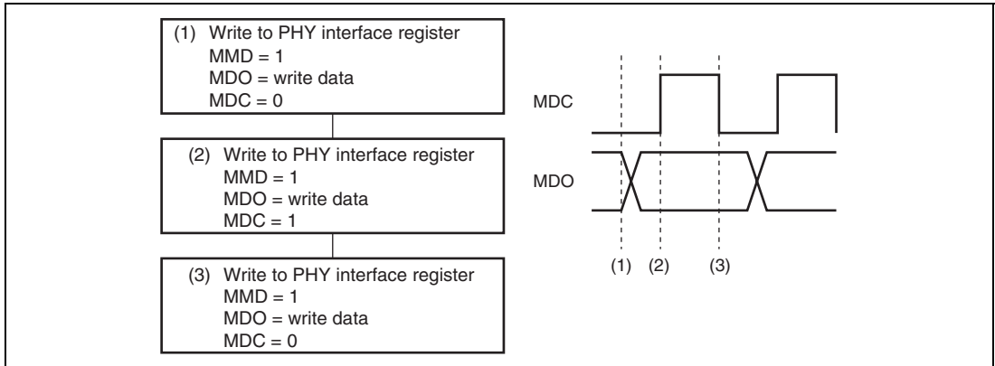
Figure 20.8 1-Bit Data Write Flowchart
