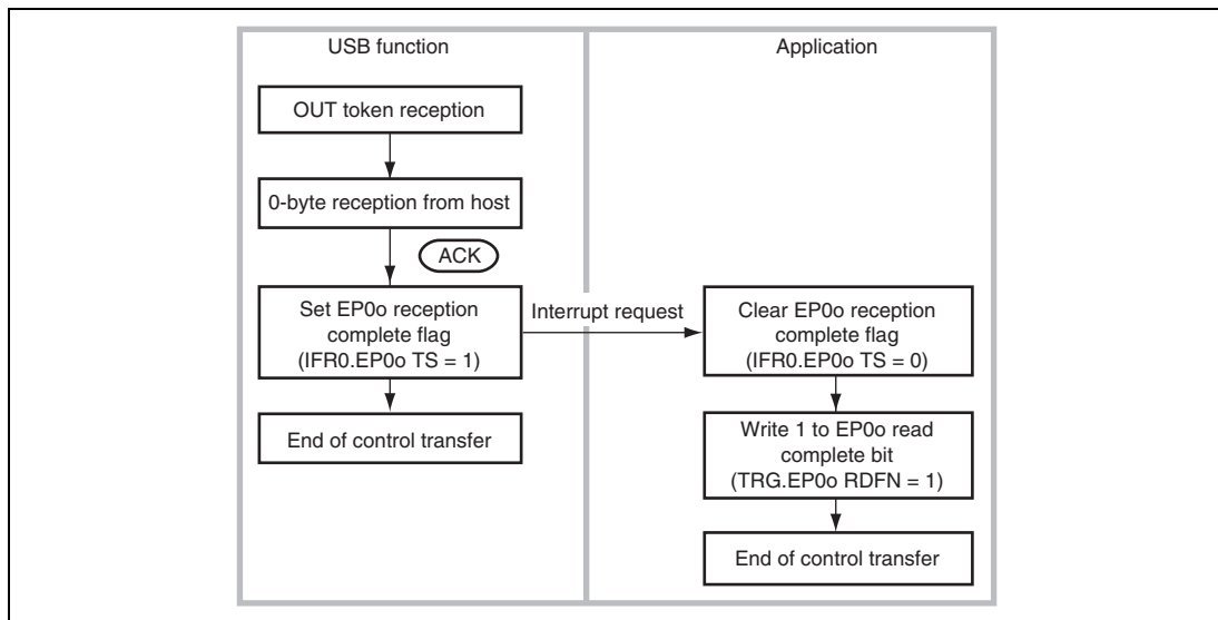
Figure 22.13 Status Stage (Control-In) Operation
