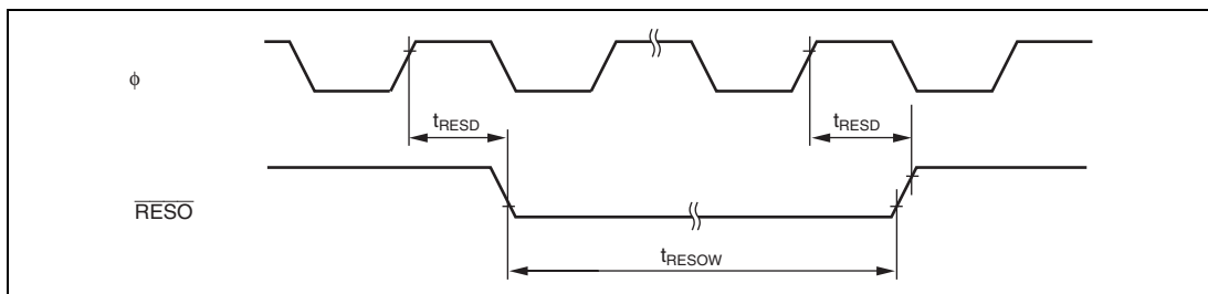
Figure 31.27 WDT Output Timing ( \overline{\text{RESO}} )
