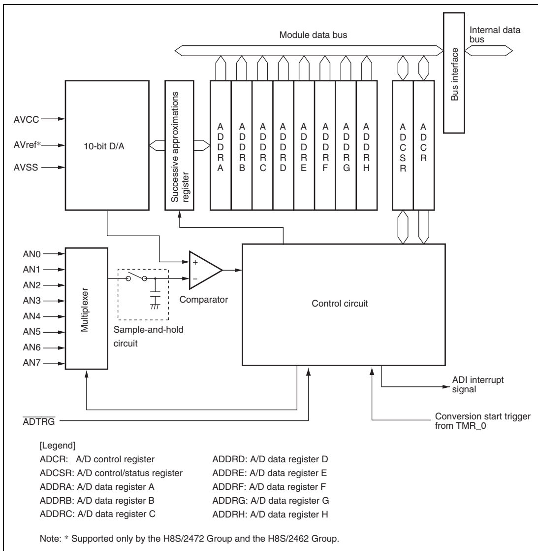
Figure 23.1 Block Diagram of the A/D Converter
