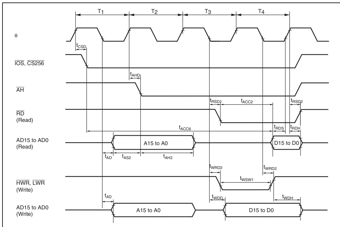
Figure 31.20 Multiplex Bus Timing/Data 2-State Access
