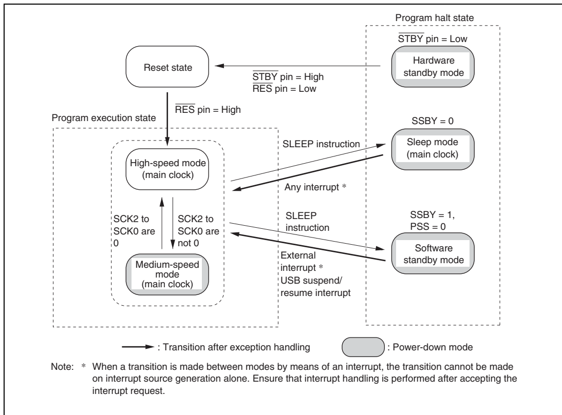
Figure 28.1 Mode Transition Diagram
