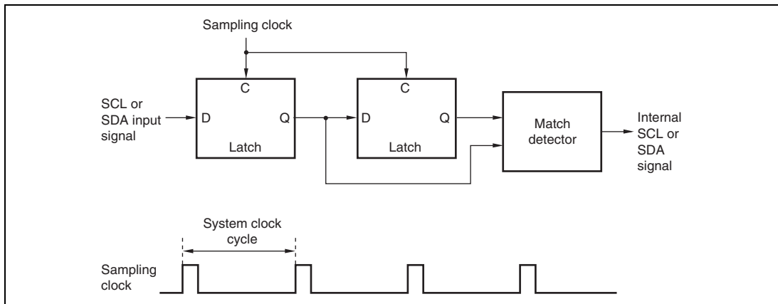
Figure 18.28 Block Diagram of Noise Canceler
