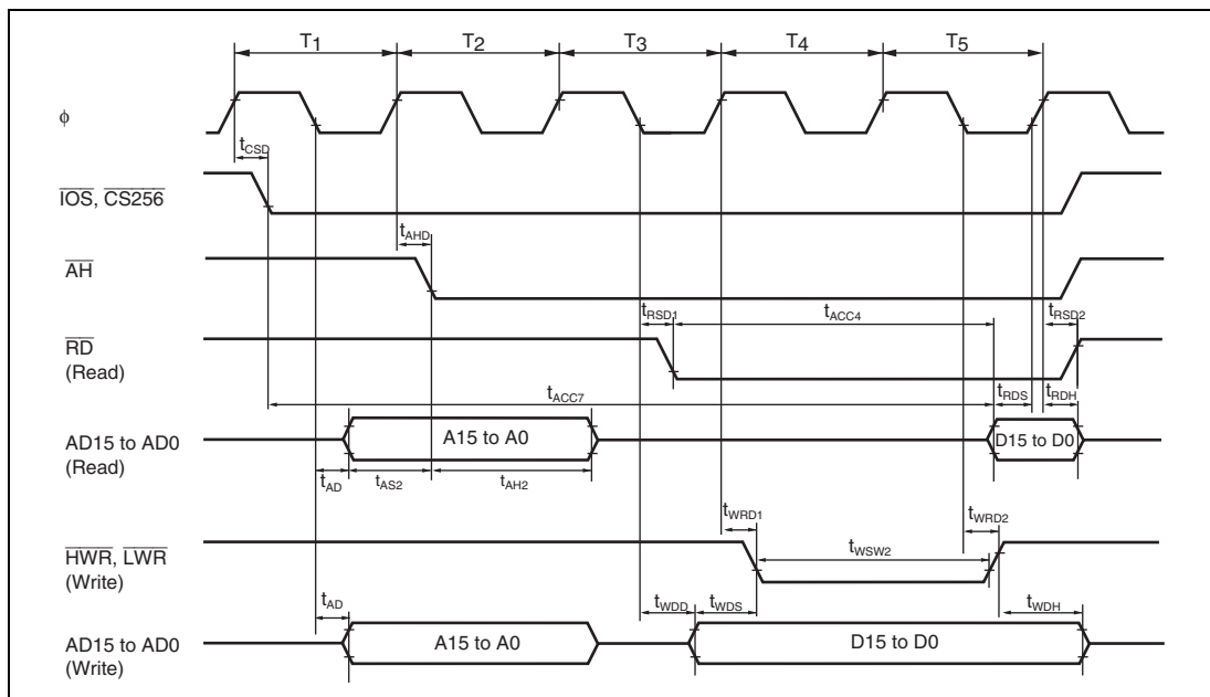
Figure 31.21 Multiplex Bus Timing/Data 3-State Access
