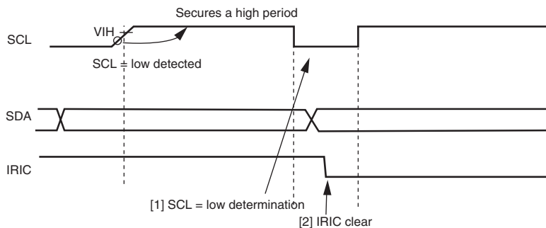
Figure 18.32 IRIC Flag Clearing Timing When WAIT = 1
