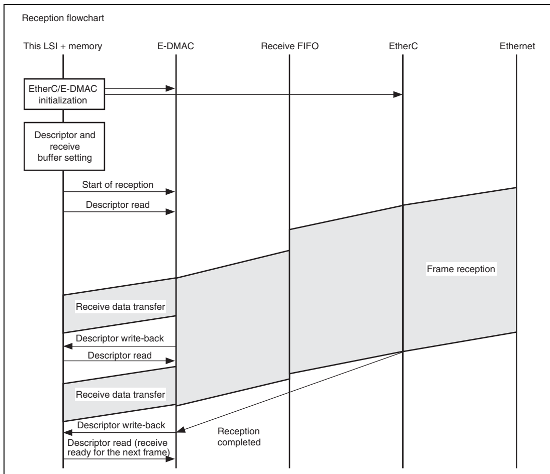
Figure 21.5 Sample Reception Flowchart
