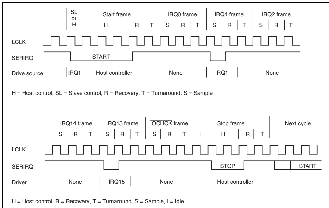
Figure 19.10 SERIRQ Timing
