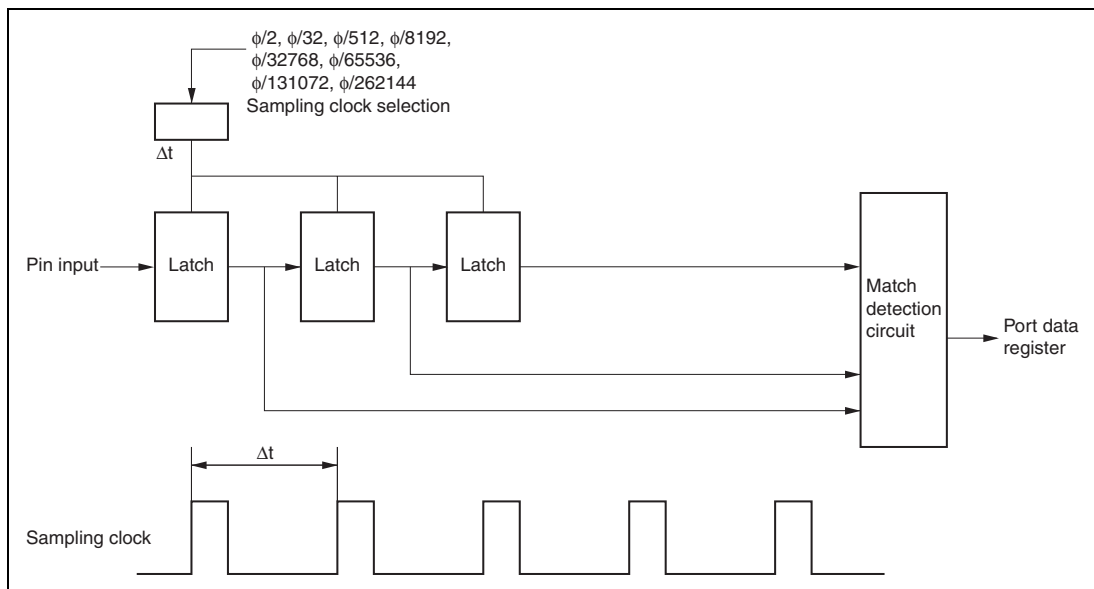
Figure 8.7 Noise Canceler Circuit
