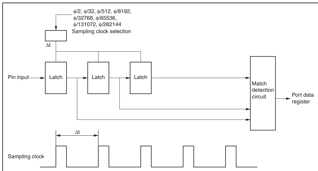
Figure 8.5 Noise Canceler Circuit
