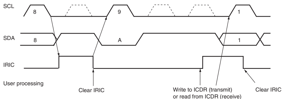
Figure 18.26 IRIC Setting Timing and SCL Control (2)
