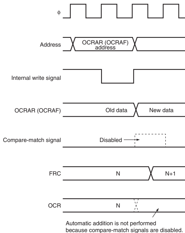
Figure 10.11 Conflict between OCR Write and Compare-Match (When Automatic Addition Function is Used)
