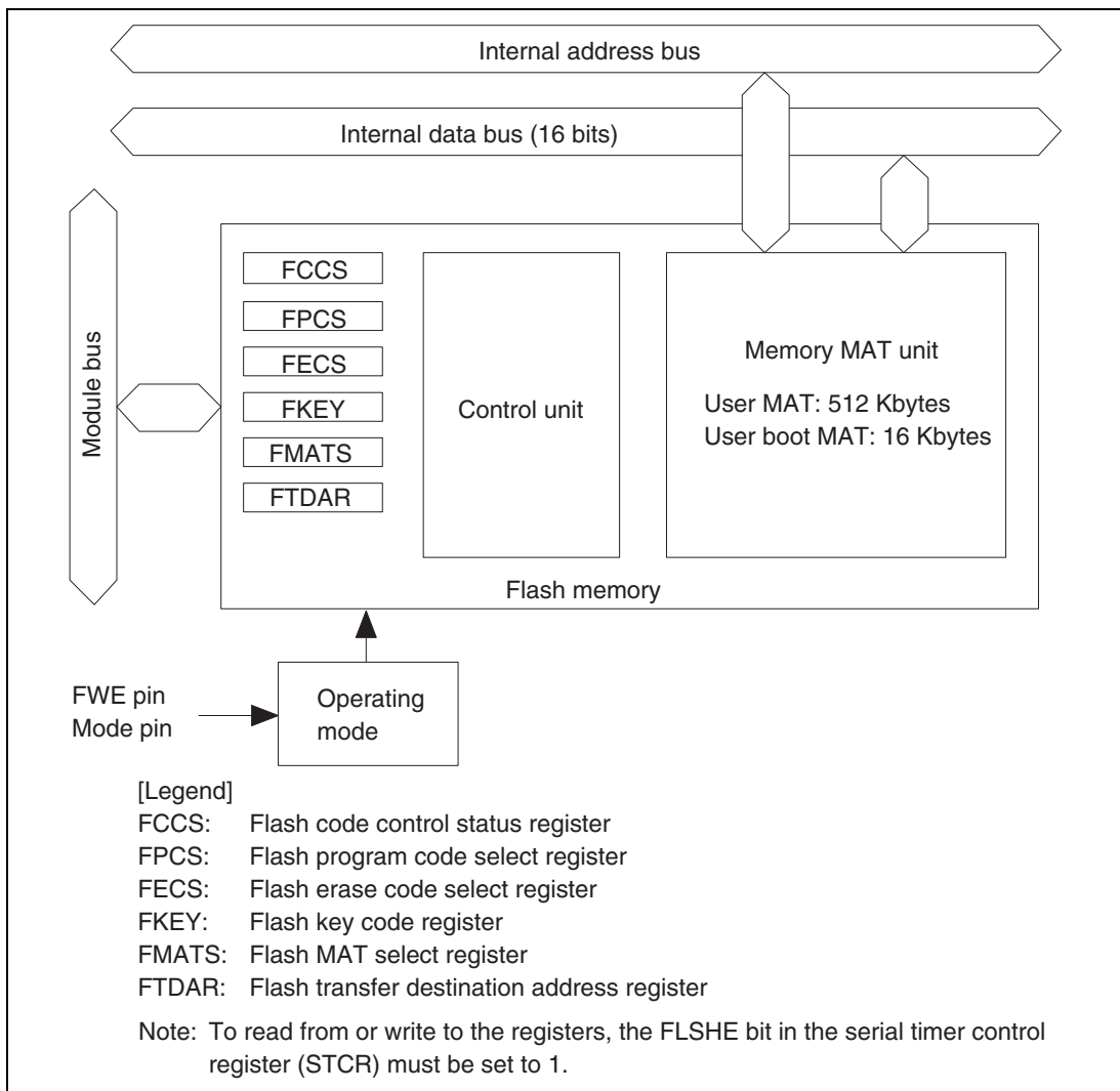
Figure 25.1 Block Diagram of Flash Memory
