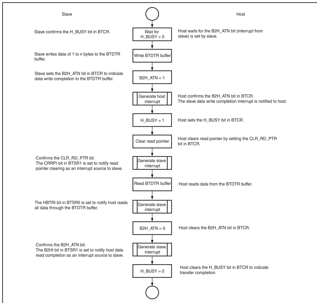
Figure 19.7 BT Read Transfer Flow
