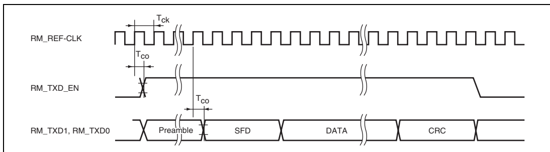
Figure 31.35 RMII Transmit Timing
