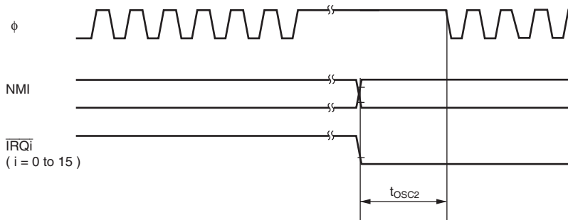
Figure 31.6 Oscillation Stabilization Timing (Exiting Software Standby Mode)
