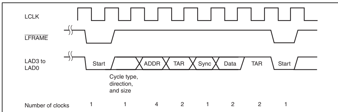
Figure 19.2 Typical \overline{\text{LFRAME}} Timing
