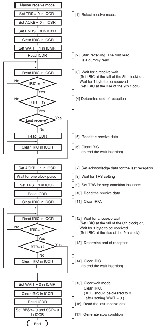
Figure 18.13 Sample Flowchart for Operations in Master Receive Mode (receiving multiple bytes) (WAIT = 1)
