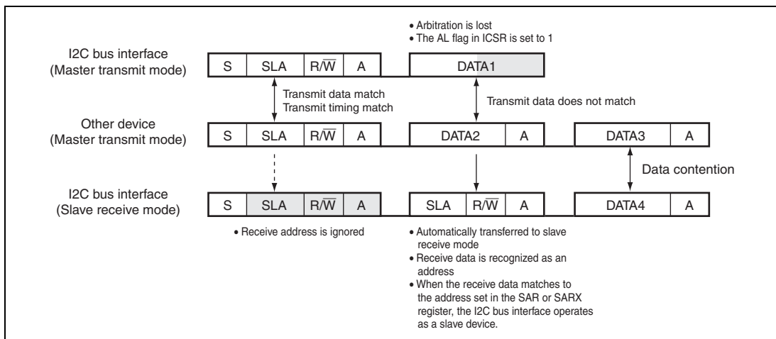
Figure 18.35 Diagram of Erroneous Operation when Arbitration Lost
