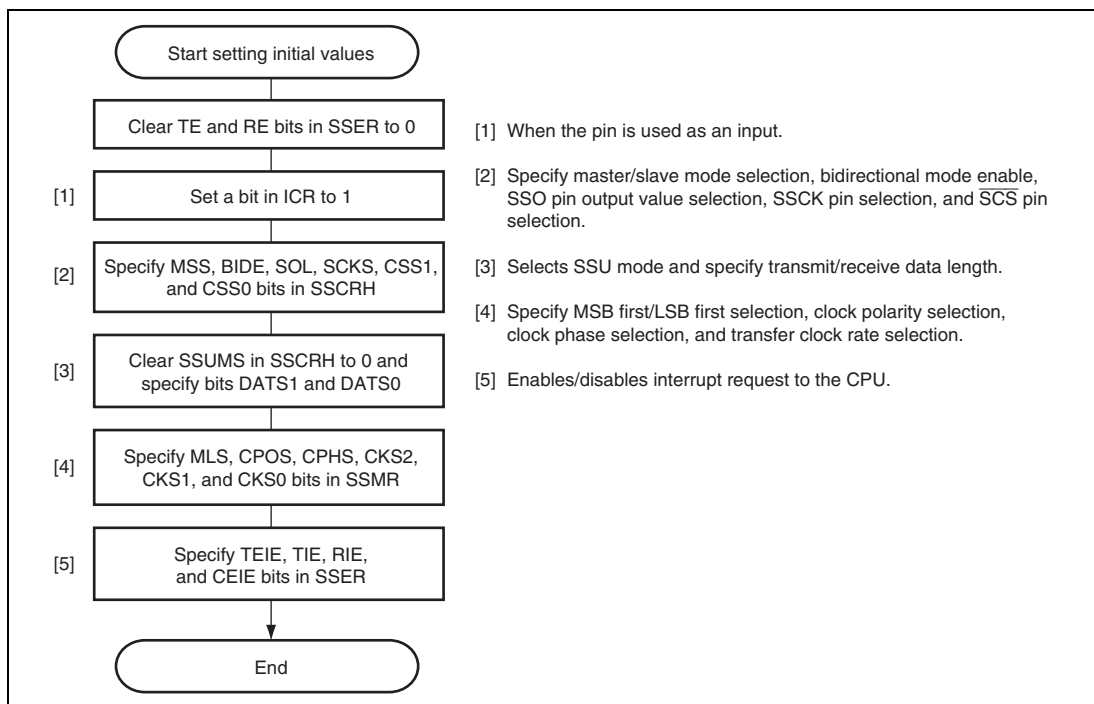
Figure 17.4 Example of Initial Settings in SSU Mode
