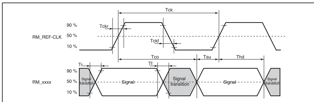
Figure 31.34 Timing of RM_REF-CLK and RMII Signals
