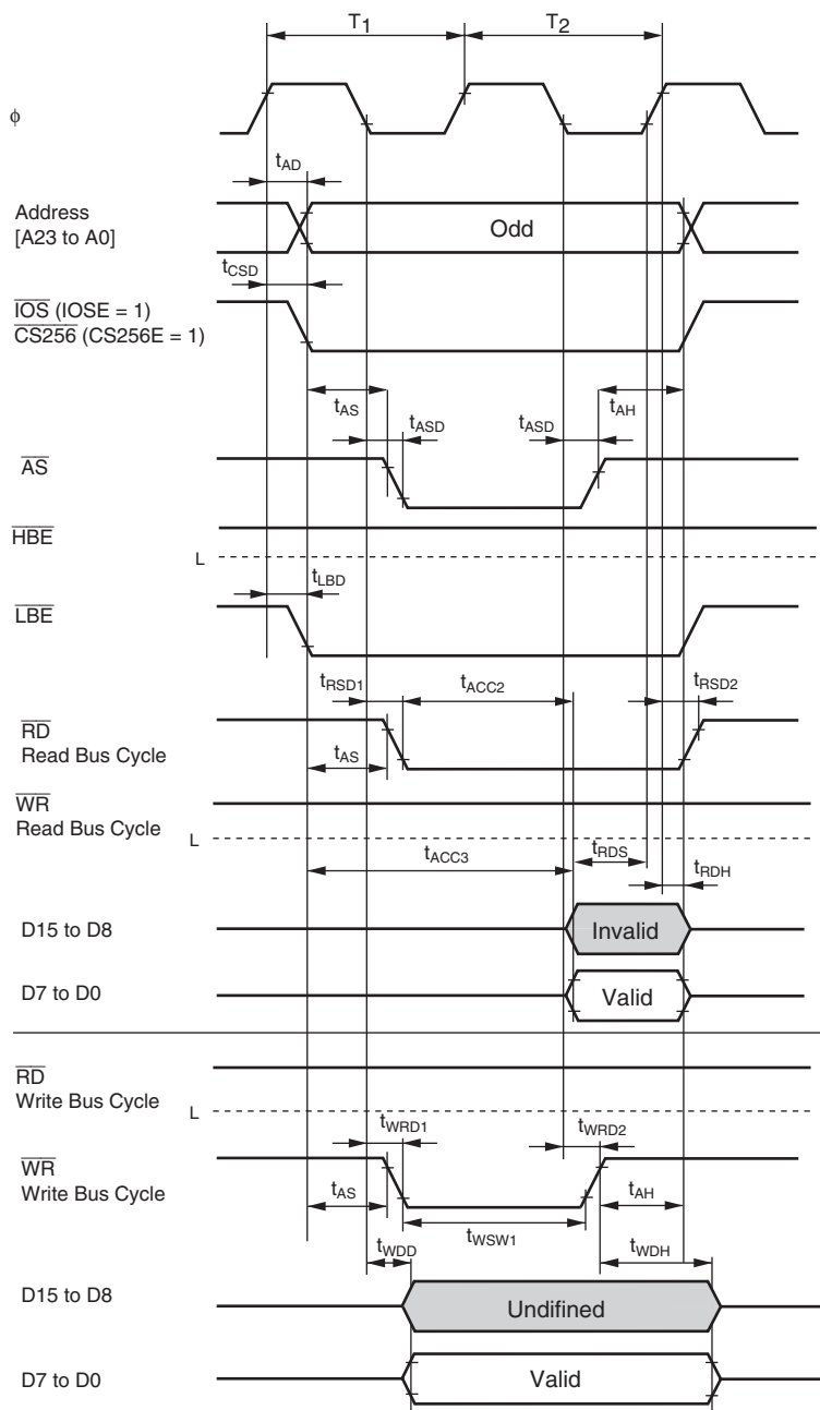
Figure 31.16 Odd Byte Access ( ADMXE = 0 )
