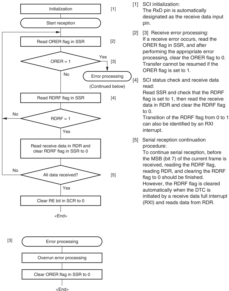
Figure 13.19 Sample Serial Reception Flowchart
