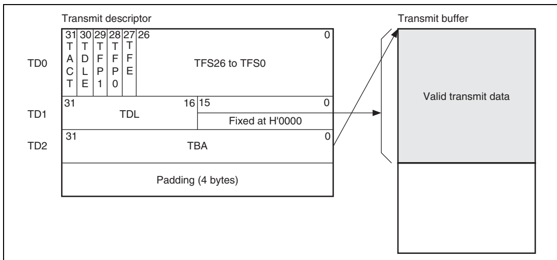
Figure 21.2 Relationship between Transmit Descriptor and Transmit Buffer
