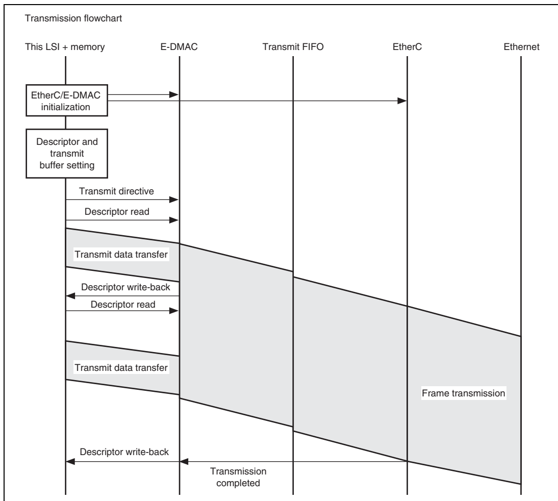
Figure 21.4 Sample Transmission Flowchart
