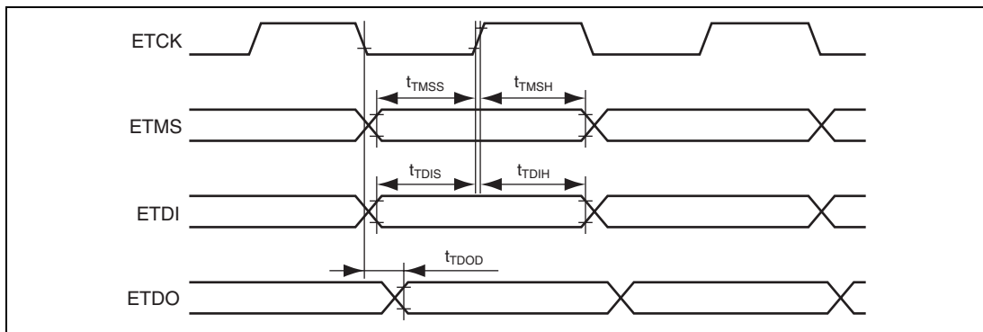
Figure 31.45 JTAG Input/Output Timing
