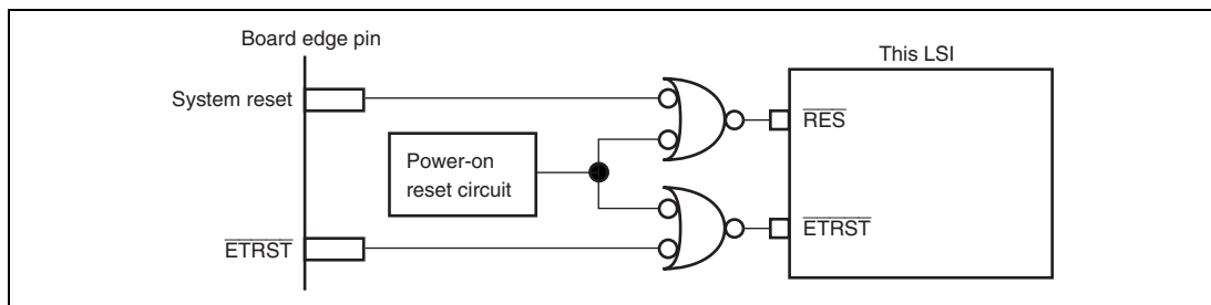
Figure 26.3 Reset Signal Circuit Without Reset Signal Interference
