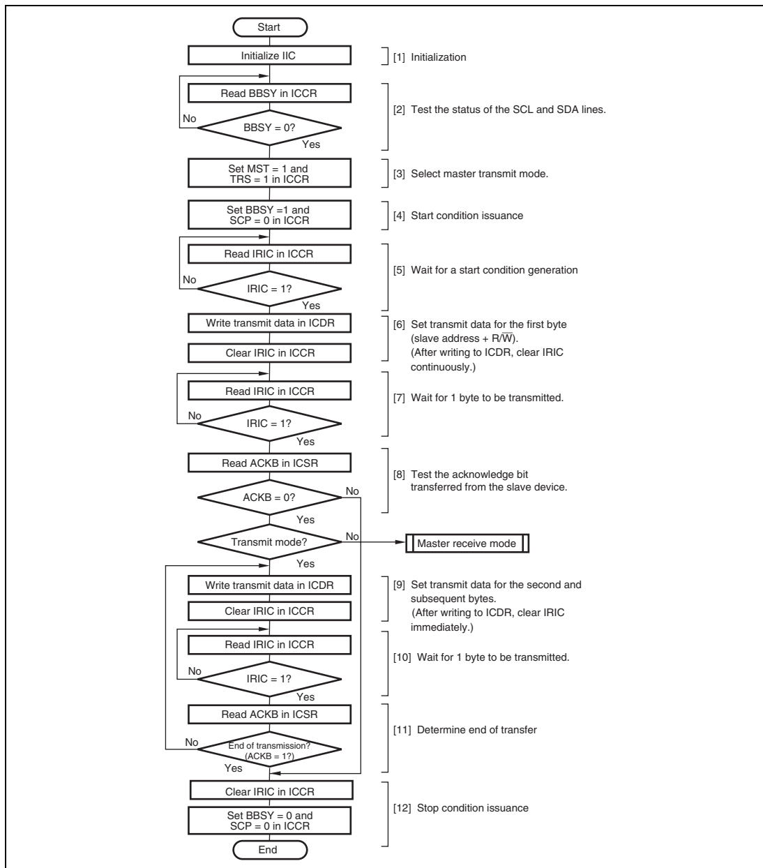
Figure 18.7 Sample Flowchart for Operations in Master Transmit Mode
