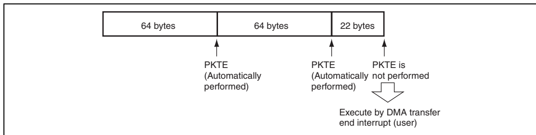
Figure 22.21 PKTE Bit Operation for EP2
