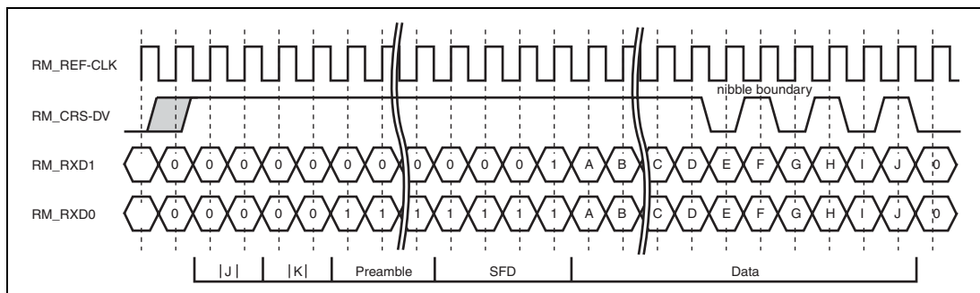
Figure 20.5 RMII Frame Receive Timing (Normal Reception)
