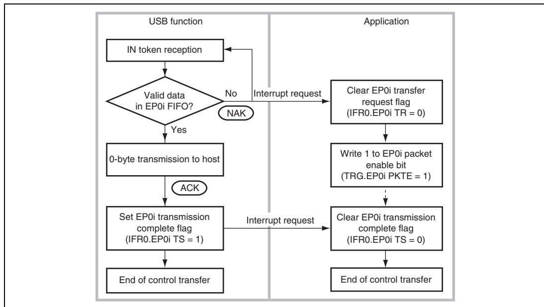
Figure 22.14 Status Stage (Control-Out) Operation
