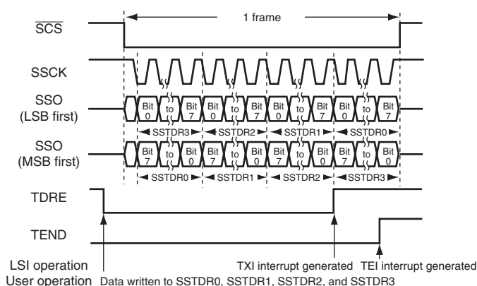
Figure 17.5 Example of Transmission Operation (SSU Mode)
