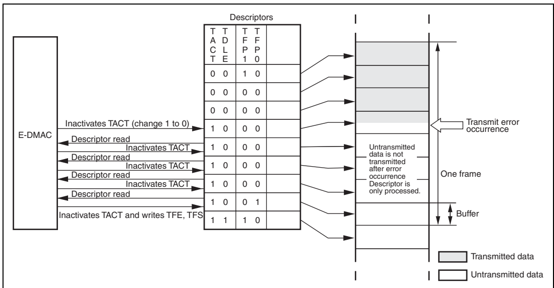
Figure 21.6 E-DMAC Operation after Transmit Error
