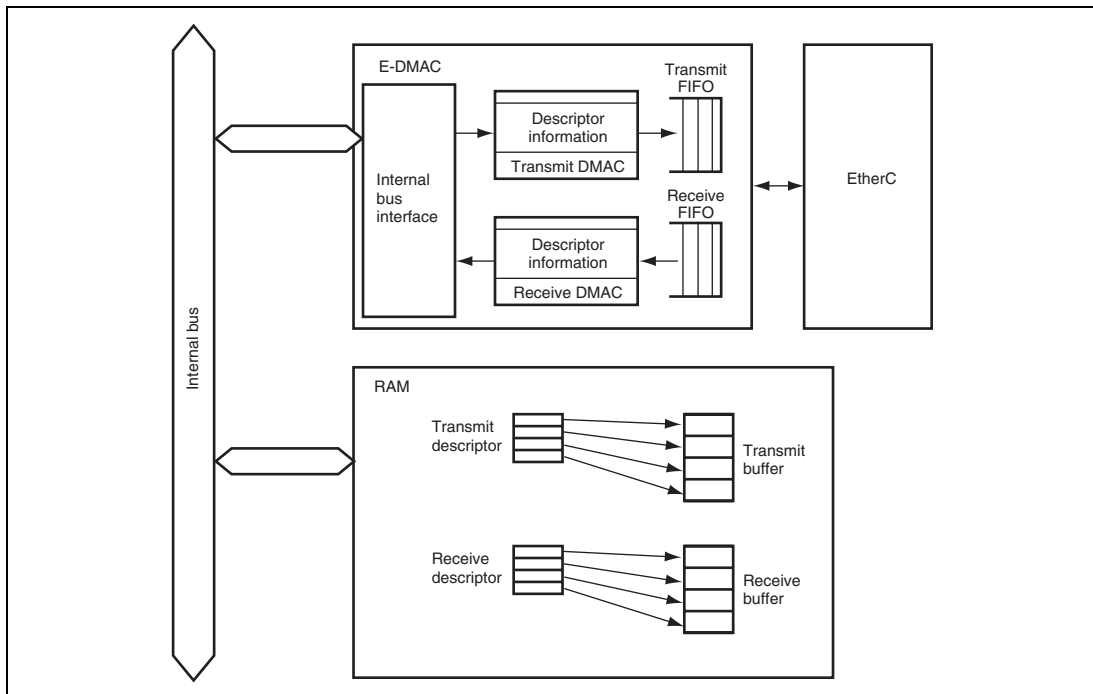
Figure 21.1 Configuration of E-DMAC, and Descriptors and Buffers
