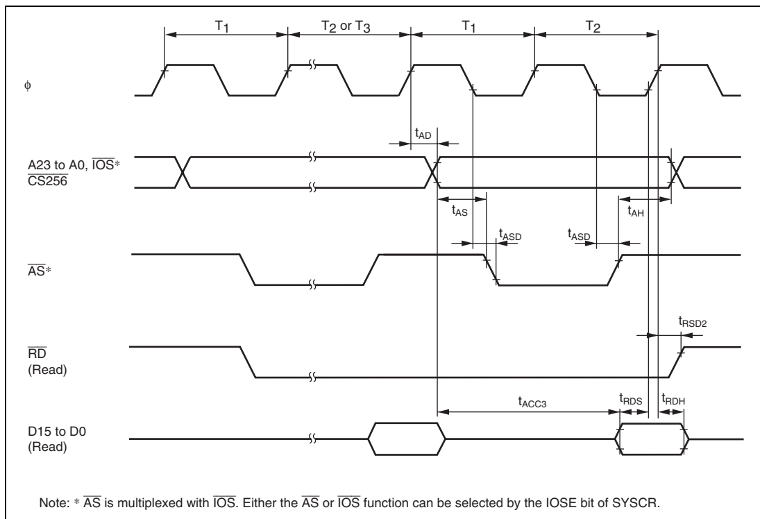
Figure 31.18 Burst ROM Access Timing/2-State Access
