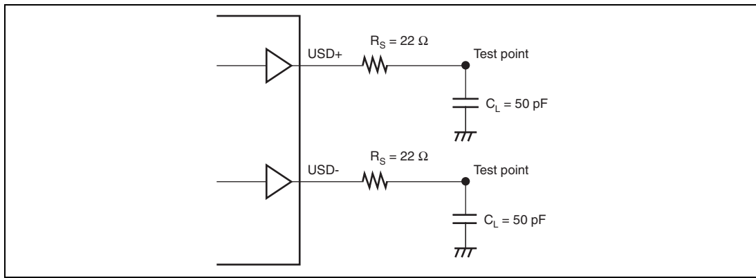
Figure 31.42 Load Condition
