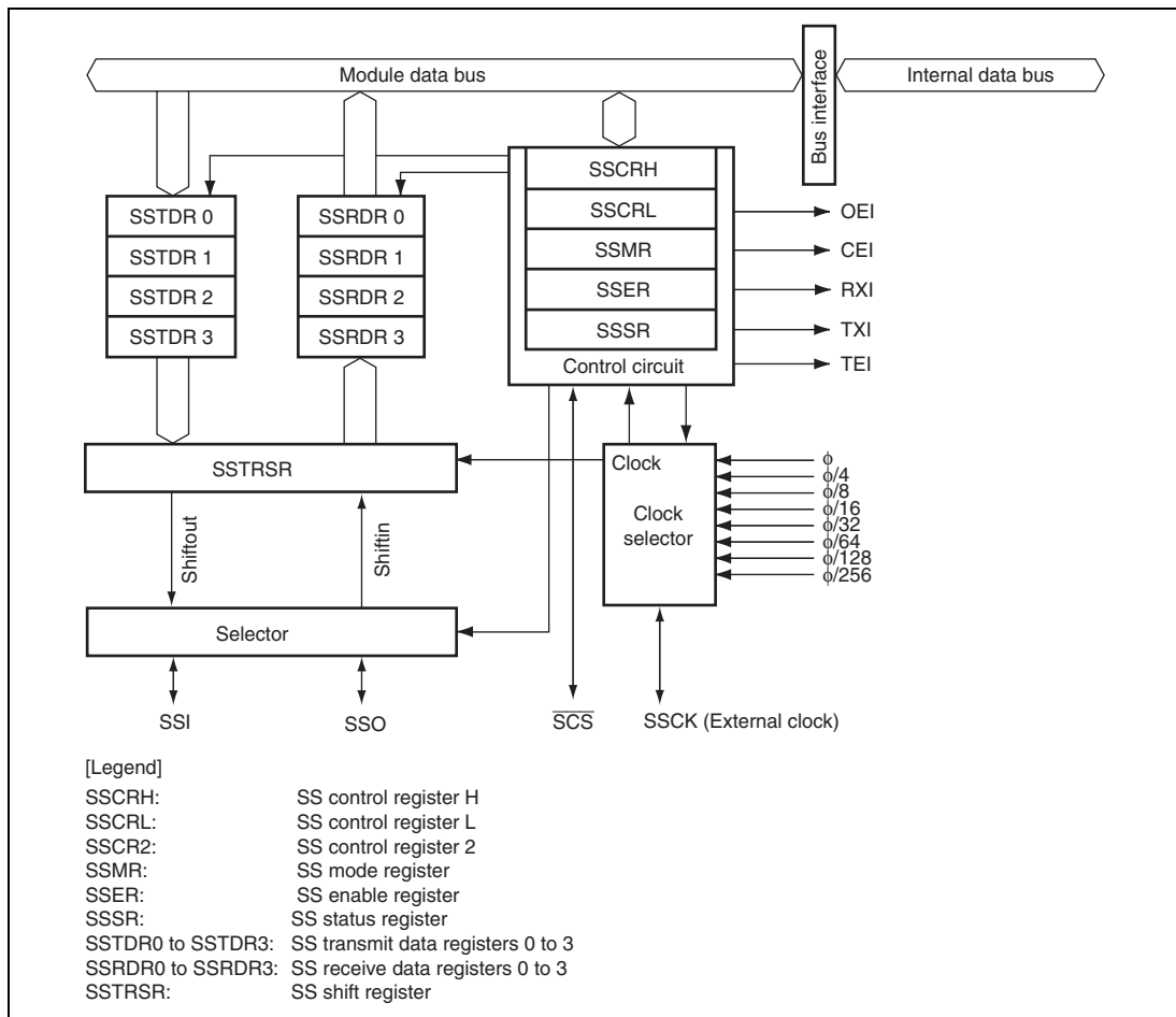
Figure 17.1 Block Diagram of SSU
