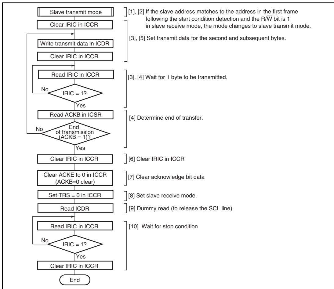
Figure 18.23 Sample Flowchart for Slave Transmit Mode
