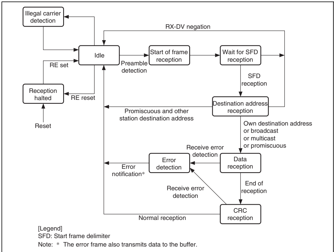
Figure 20.3 EtherC Receiver State Transmissions
