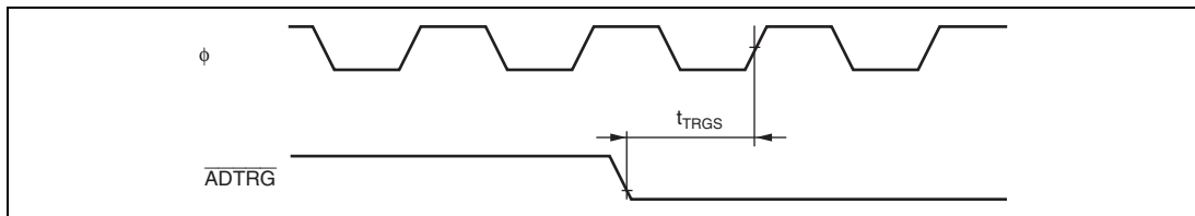
Figure 31.26 A/D Converter External Trigger Input Timing
