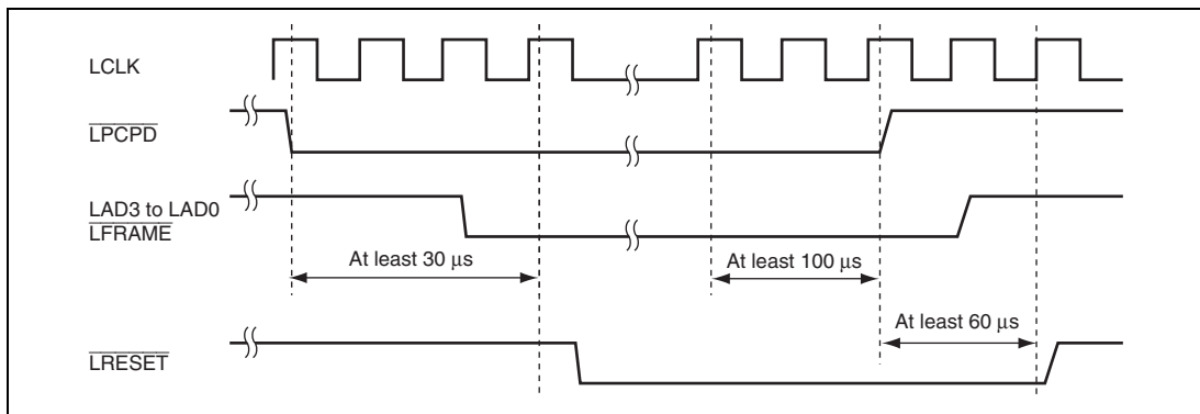
Figure 19.9 Power-Down State Termination Timing
