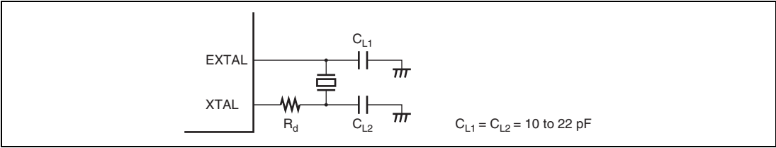
Figure 27.2 Typical Connection to Crystal Resonator
