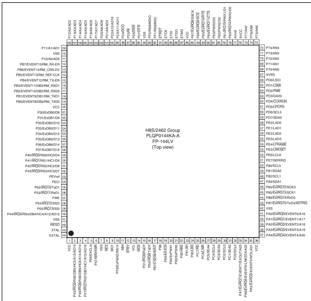
Figure 1.4 Pin Assignments (H8S/2462 Group)
