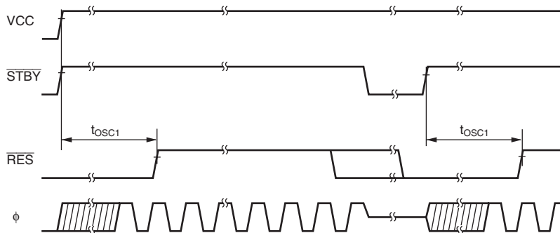
Figure 31.5 Oscillation Stabilization Timing
