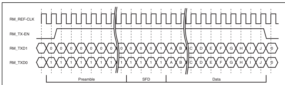
Figure 20.4 RMII Frame Transmit Timing (Normal Transmission)
