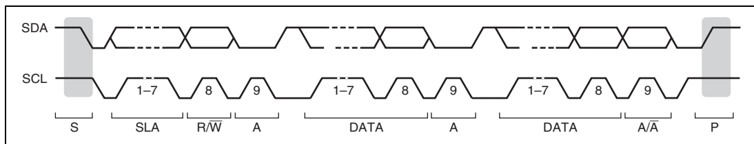
Figure 18.5 I 2 C Bus Timing
