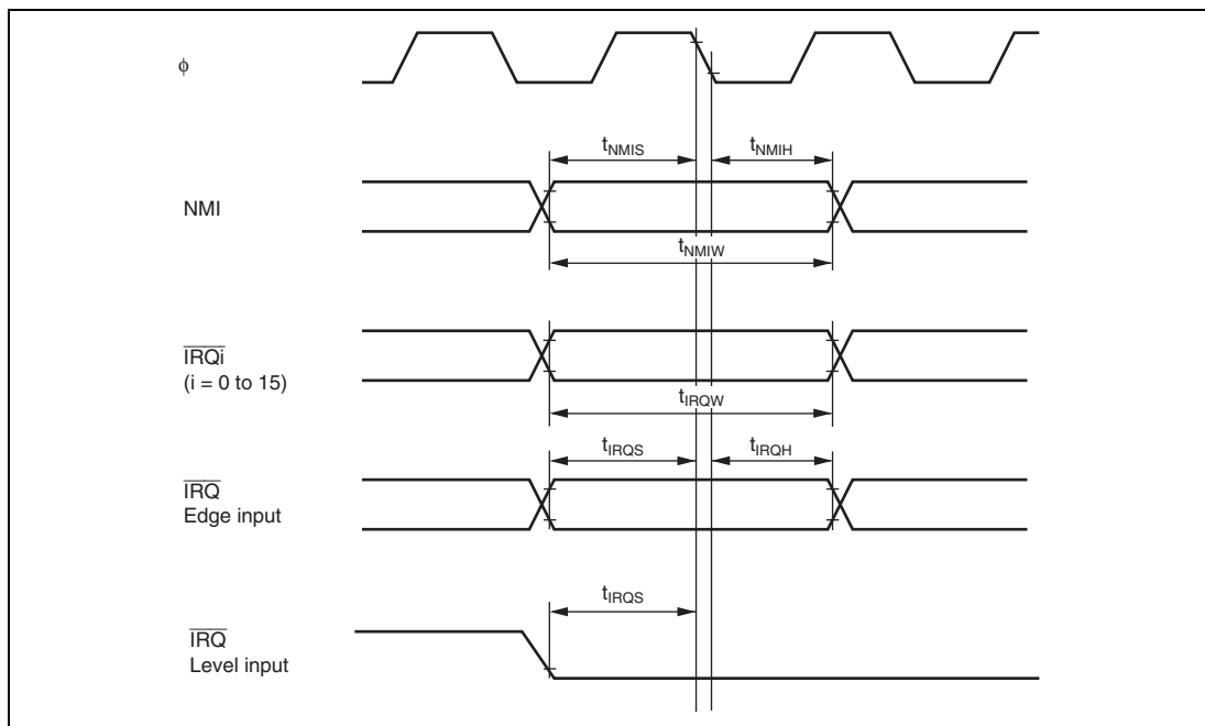
Figure 31.11 Interrupt Input Timing
