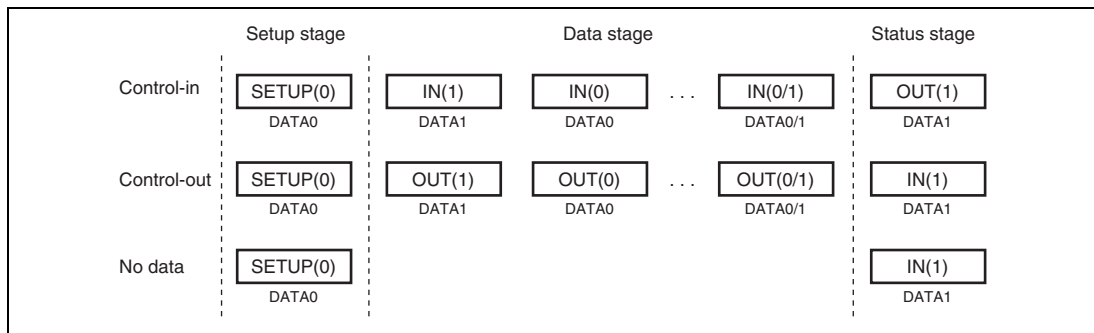
Figure 22.9 Transfer Stages in Control Transfer
