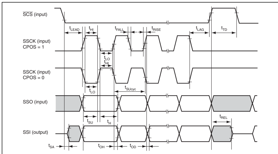
Figure 31.31 SSU Timing (Slave, CPHS = 0)
