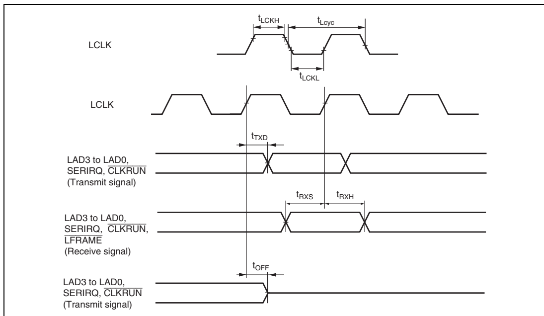
Figure 31.33 LPC Interface (LPC) Timing
