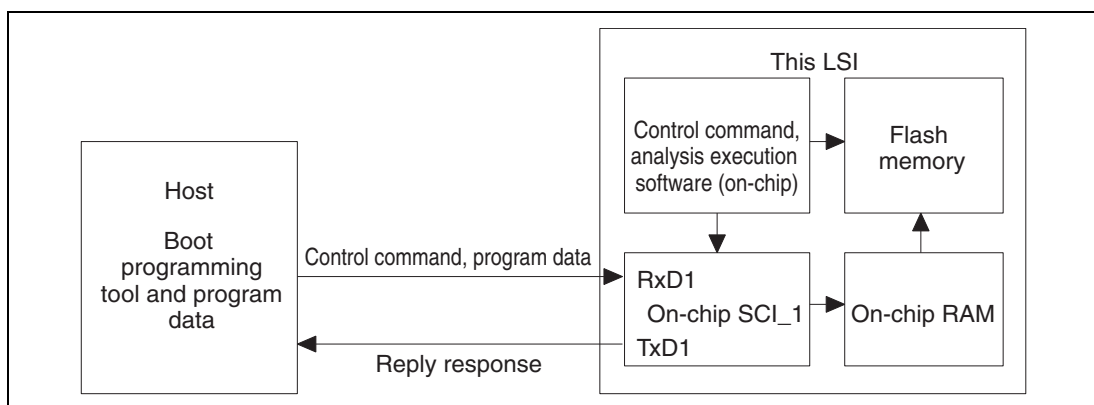
Figure 25.6 System Configuration in Boot Mode
