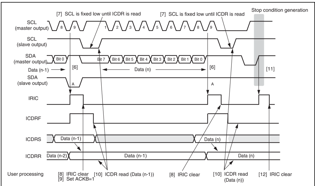
Figure 18.19 Slave Receive Mode Operation Timing Example (2) (MLS = 0, HNDS= 1)
