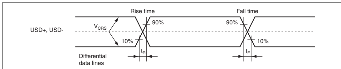
Figure 31.41 Data Signal Timing
