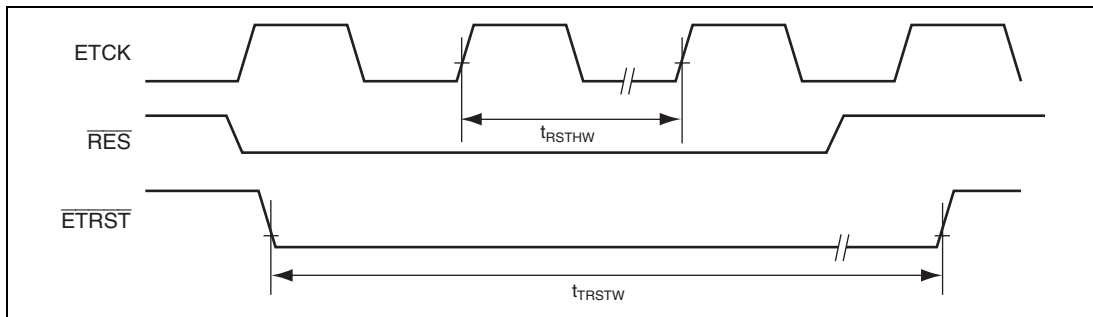
Figure 31.44 Reset Hold Timing
