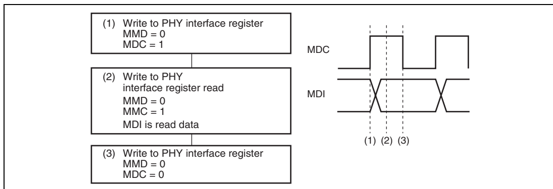
Figure 20.10 1-Bit Data Read Flowchart
