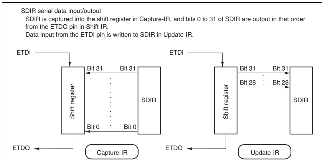
Figure 26.4 Serial Data Input/Output (1)
