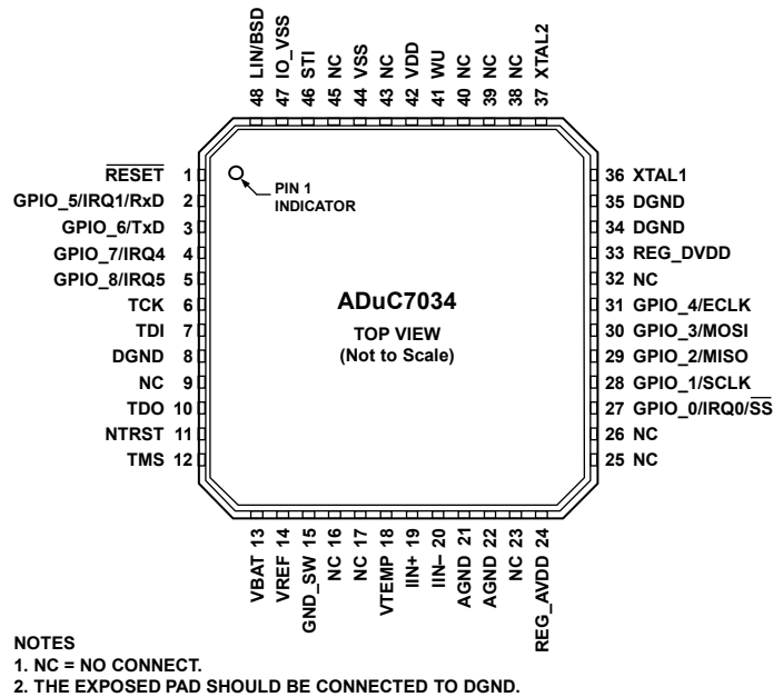
Figure 7. Pin Configuration
