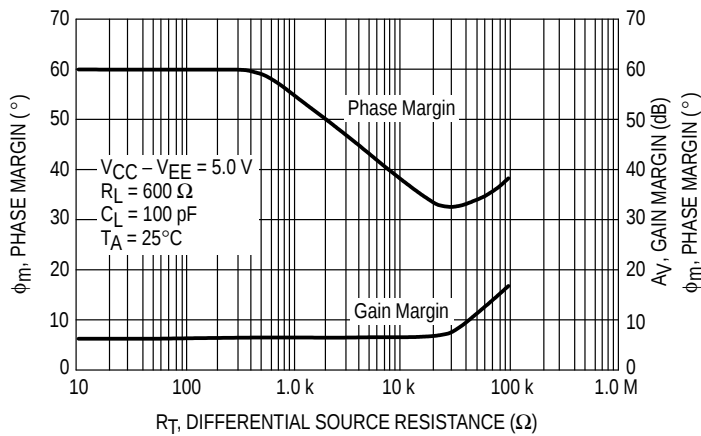
Figure 24. Gain and Phase Margin versus Differential Source Resistance
