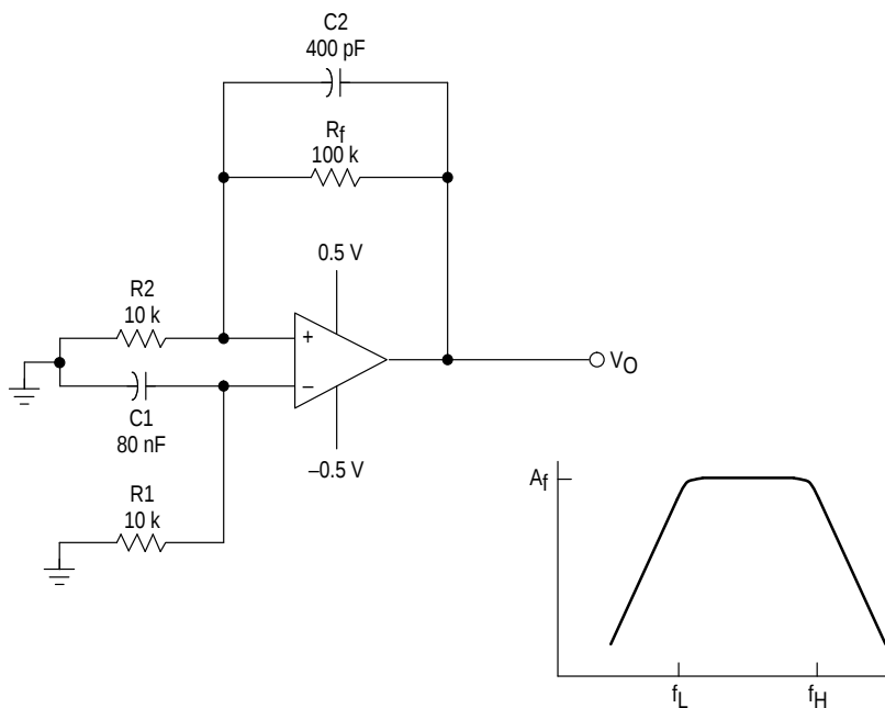
Figure 33. 1.0 V Voiceband Filter
