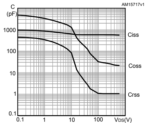
Figure 10. Capacitance variations
