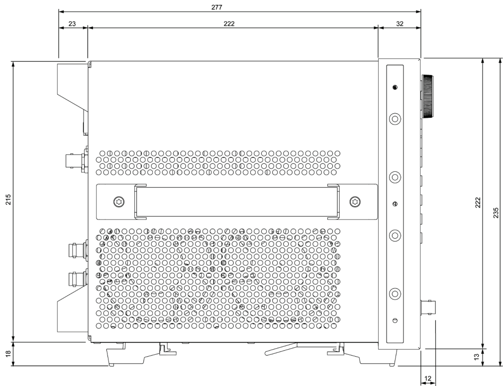
Figure 12. Side view (Millimeters)
