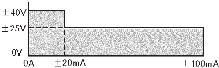
Figure 1. DC bias range
