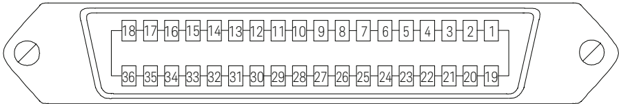
Figure 8. 24 bit I/O port pin assignment
