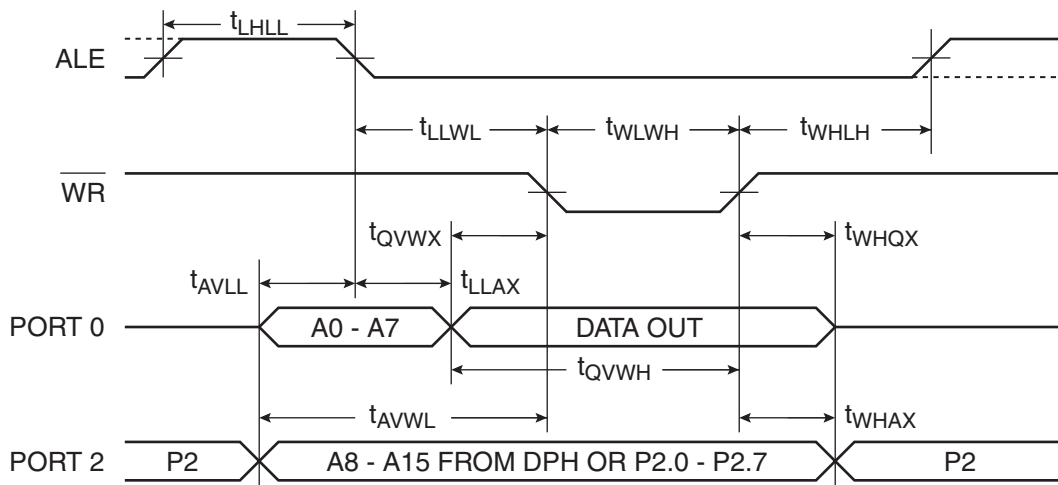
Figure 18-8. External Data Memory Write Cycle
