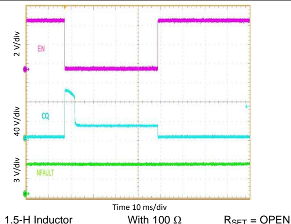
Figure 29. CQ Driving, Low Side Mode
