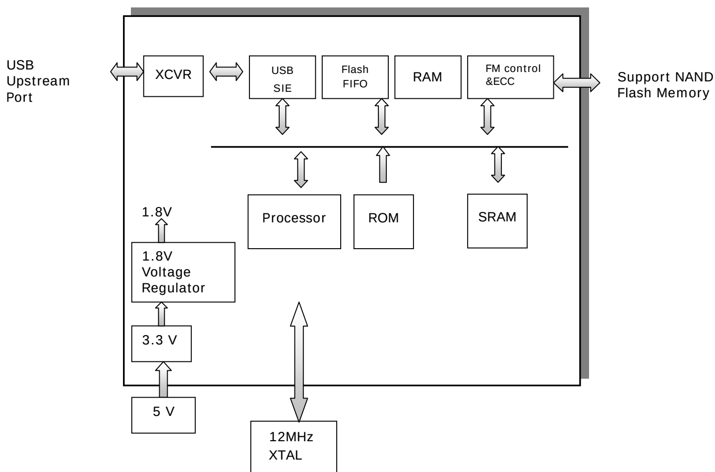
Figure 4.1 AU9387 Block Diagram
