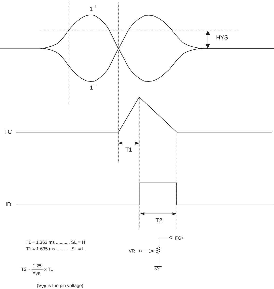
Index Delay Pulse Timing Chart
