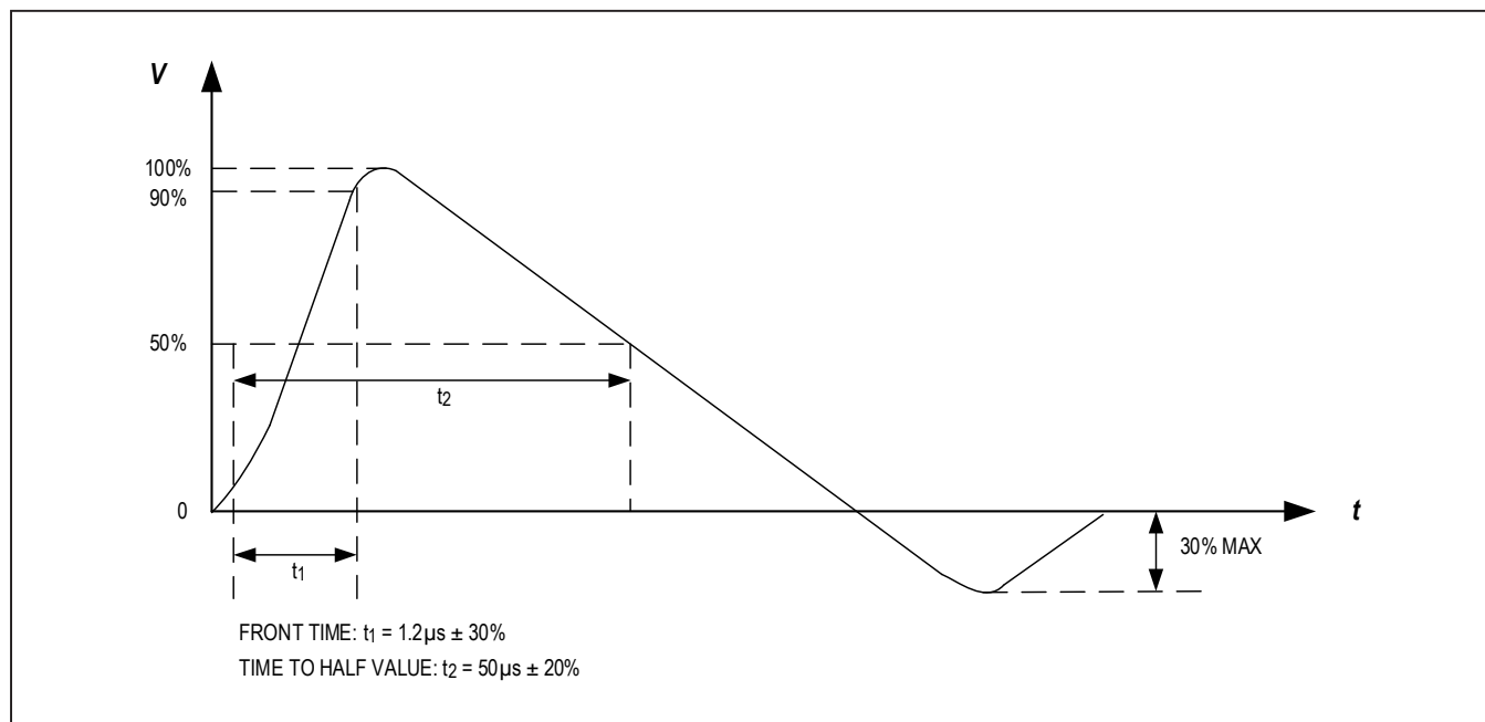
Figure 8. 1.2/50 \mu\text{s} Surge Voltage Waveform
