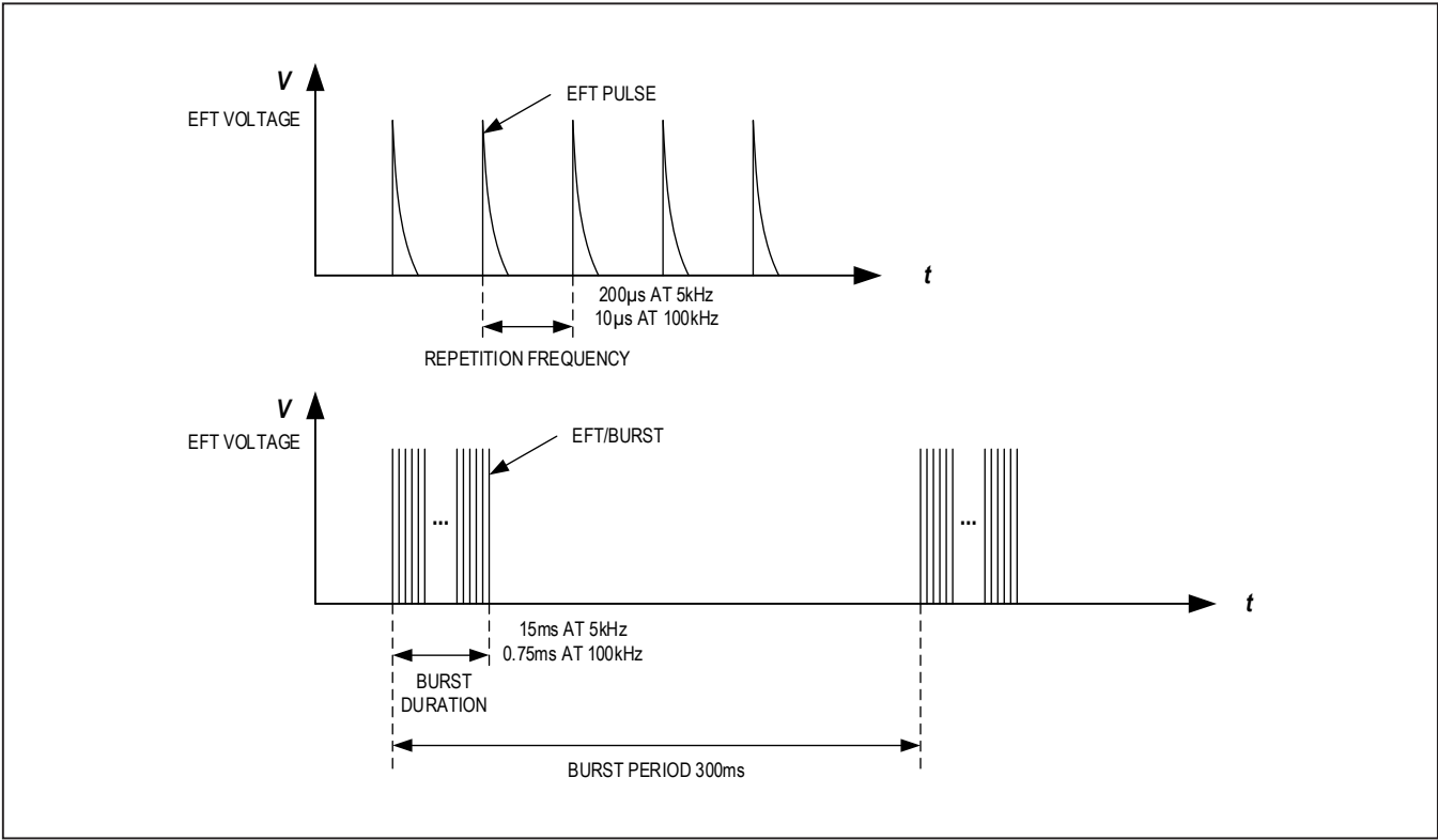
Figure 7. Electrical Fast Transient/Burst Waveform
