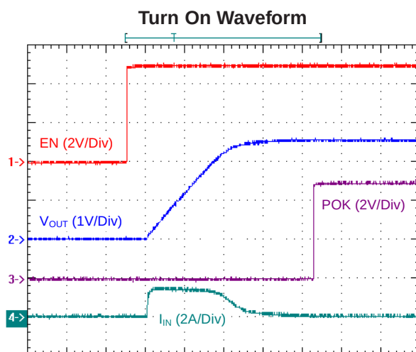
Time : 400us/Div V_{CNTL} = 5V , V_{IN} = 3.3V , C_{OUT} = 470\mu F , No Load
