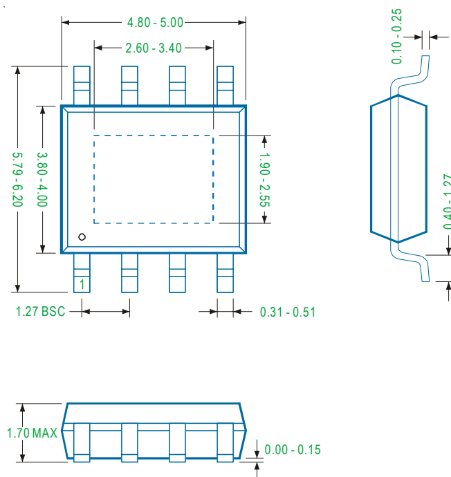
PSOP-8L
