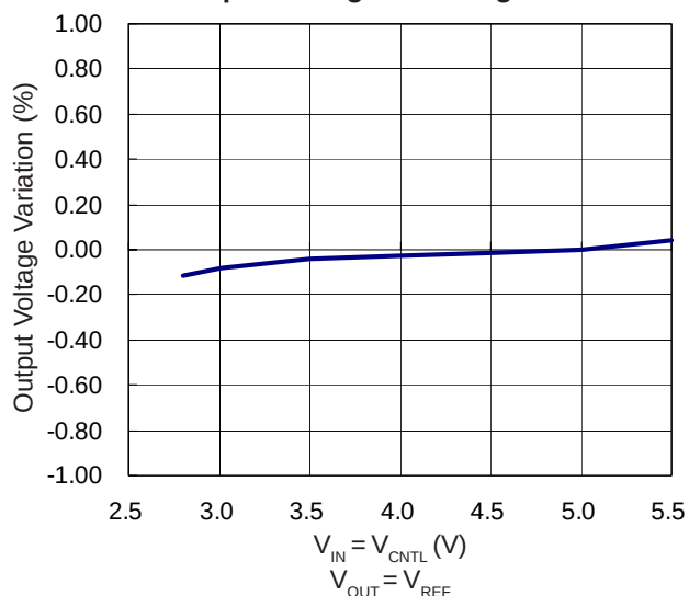
Output Voltage Line Regulation
