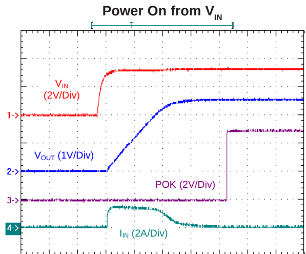
Time : 400us/Div V_{CNTL} = 5V , V_{IN} = 3.3V , C_{OUT} = 470\mu F , No Load
