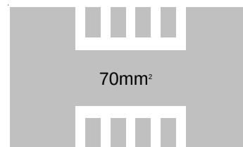
Figure 4. Copper Area of Thermal Pad = 70\text{mm}^2 , \theta_{JA} = 45^{\circ}\text{C/W}
