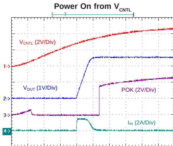
Time : 1ms/Div V_{CNTL} = 5V , V_{IN} = 3.3V , C_{OUT} = 470\mu F , No Load
