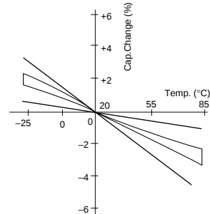
T110 (N450 \pm 300 ppm/ ^{\circ} C)
