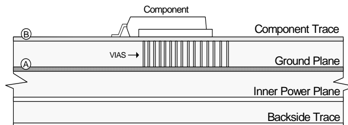
Figure 3 - Heatsink
