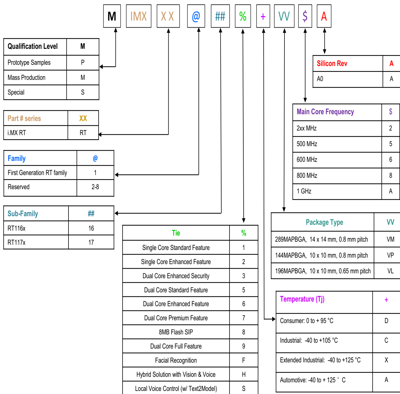
Figure 1. Part number nomenclature—i.MX RT11XX family
