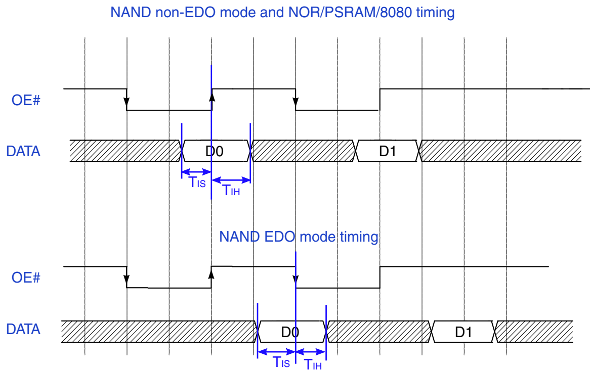
Figure 18. SEMC input timing in ASYNC mode
