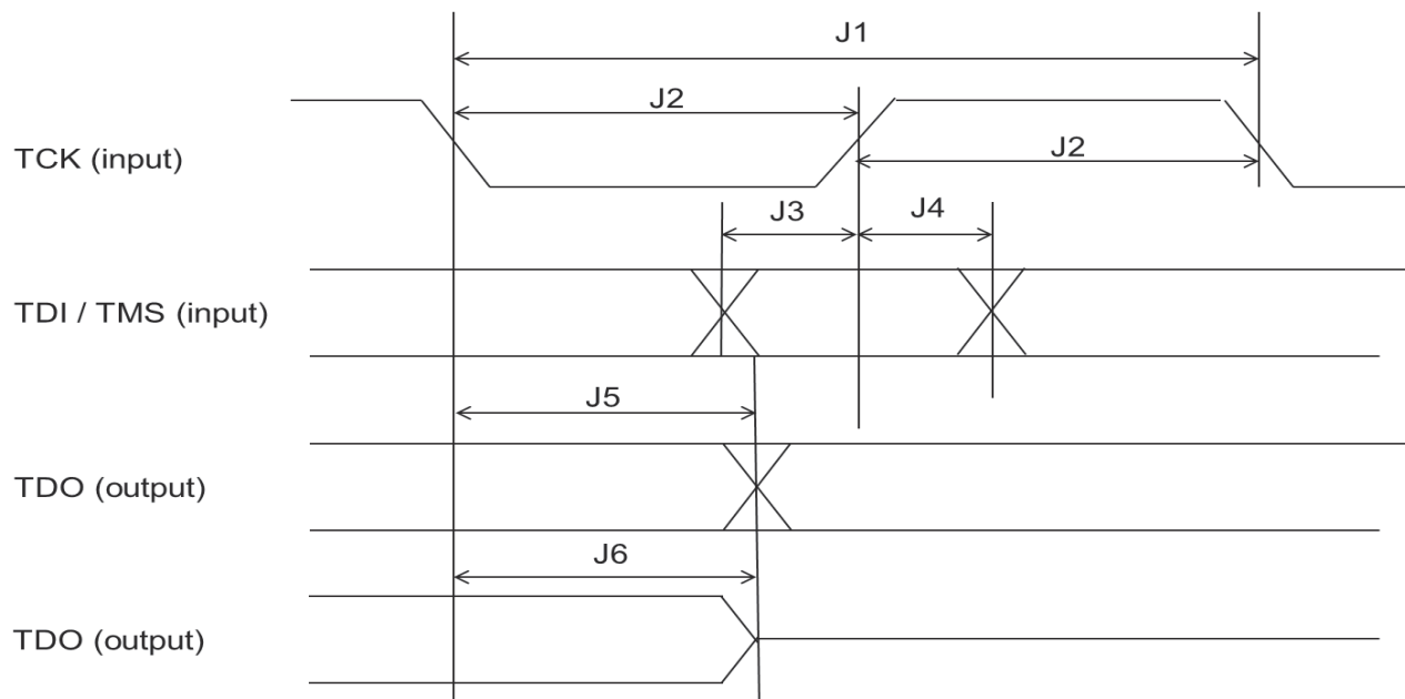
Figure 12. JTAG controller timing
