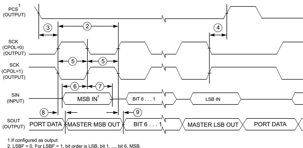
Figure 37. LPSPI Master mode timing (CPHA = 1)
