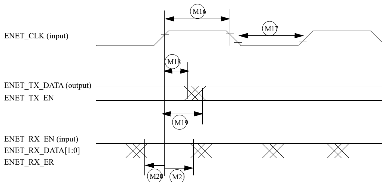
Figure 49. RMI mode signal timing diagram
