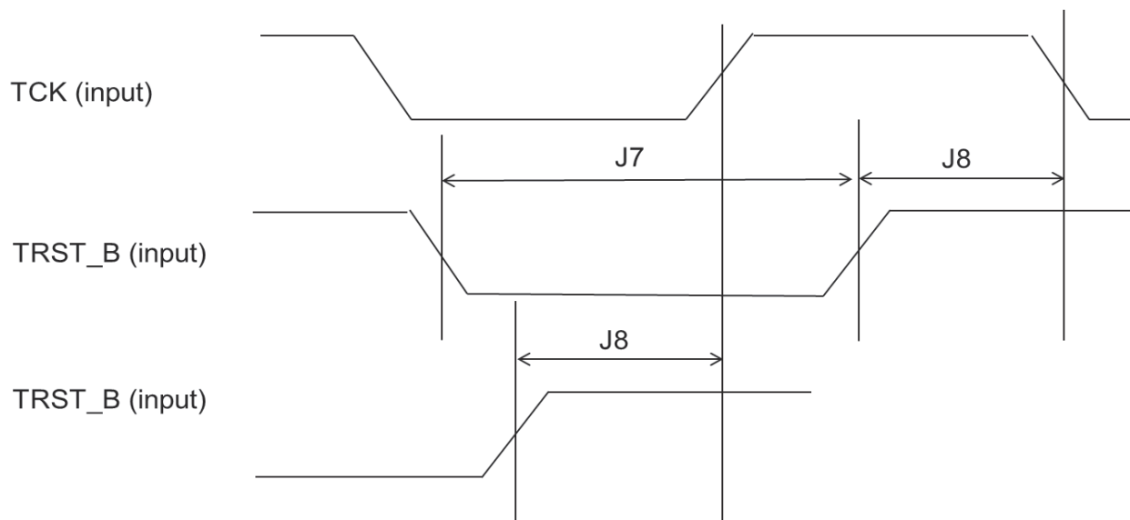
Figure 13. JTAG_TRST_B timing
