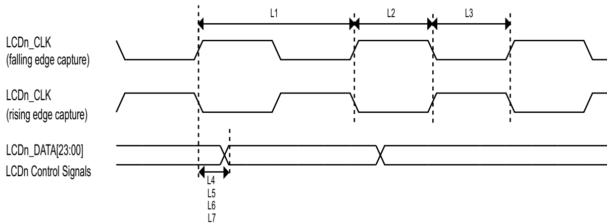
Figure 31. LCD timing
