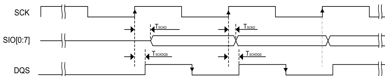
Figure 21. FlexSPI input timing in SDR mode where FlexSPIn_MCR0[RXCLKSRC] = 0X3 (case A1)
