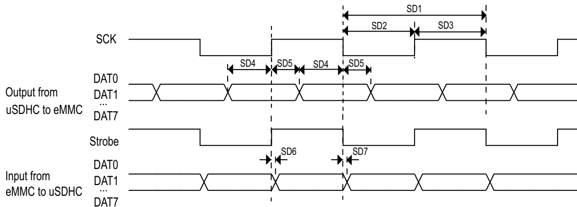
Figure 44. HS400 timing
