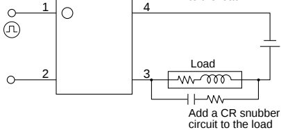
Non-latch type
