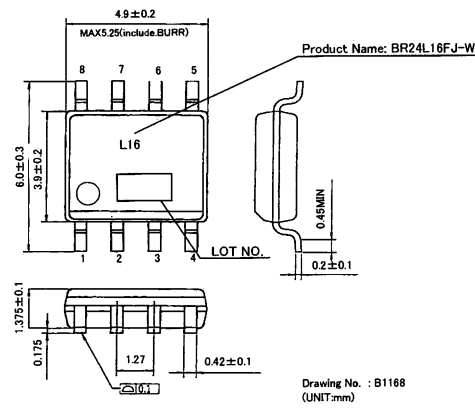
Fig.-4(b) PHYSICAL DIMENSION SOP8 (BR24L16FJ-W)
