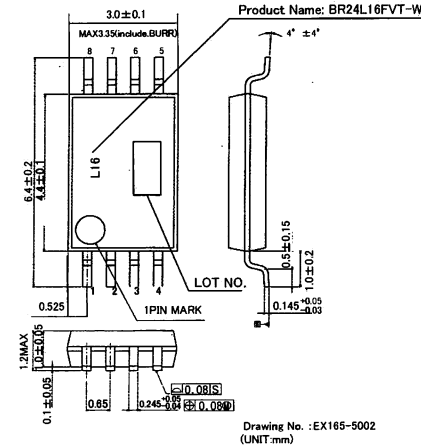
Fig.-4(d) PHYSICAL DIMENSION TSSOP-B8 (BR24L16FVT-W)
