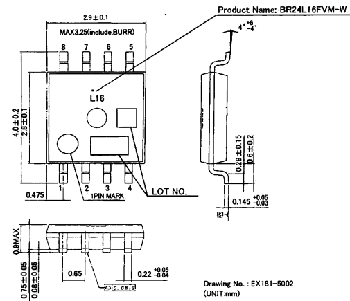
Fig.-4(e) PHYSICAL DIMENSION MSOP8 (BR24L16FVM-W)
