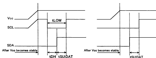
Fig.-3(b) SCL='L' and SDA='L'
