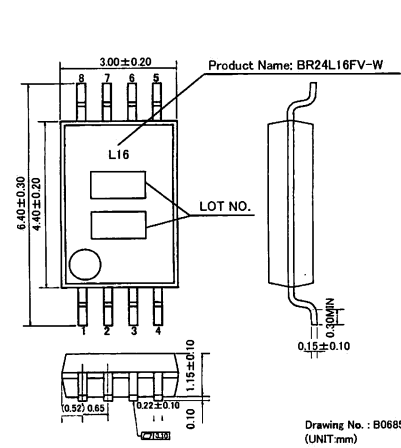
Fig.-4(c) PHYSICAL DIMENSION SSOP-B8 (BR24L16FV-W)
