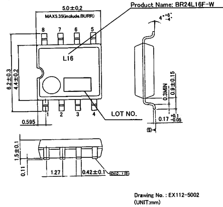
Fig.-4(a) PHYSICAL DIMENSION SOP8 (BR24L16F-W)
