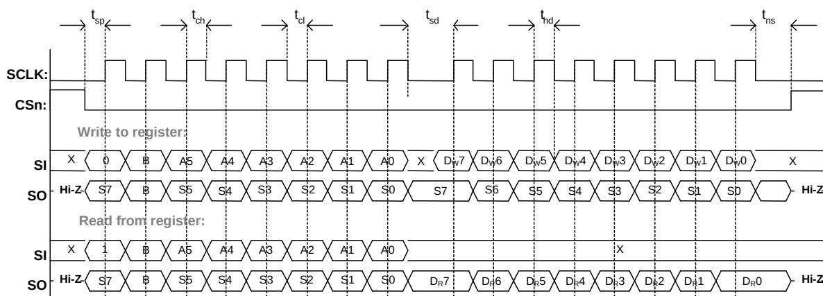
Figure 7: Configuration Registers Write and Read Operations
