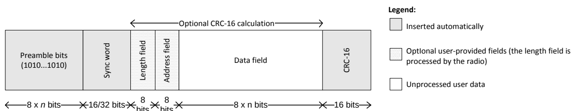
Figure 10: Packet Format
