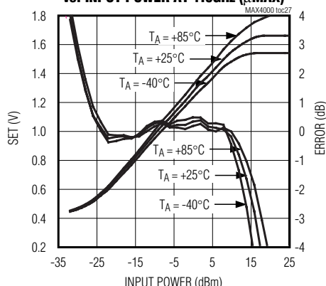
MAX4002 SET AND LOG CONFORMANCE vs. INPUT POWER AT 1.9GHz ( \mu MAX)
