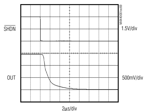
\overline{SHDN} RESPONSE TIME
