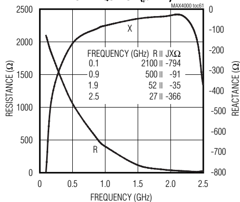
MAX4000 INPUT IMPEDANCE vs. FREQUENCY ( \mu MAX)
