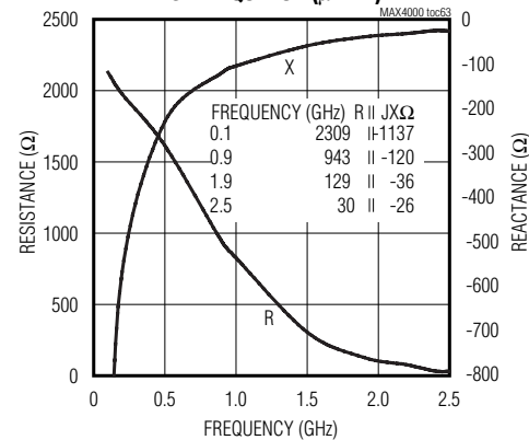
MAX4002 INPUT IMPEDANCE vs. FREQUENCY ( \mu MAX)
