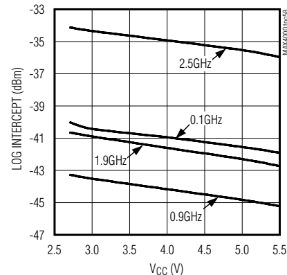
MAX4002 LOG INTERCEPT vs. V_{CC} (UCSP)
