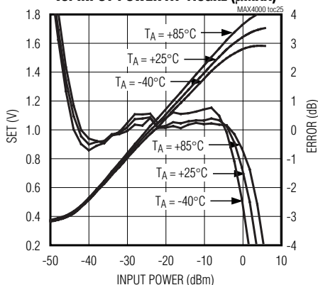
MAX4000 SET AND LOG CONFORMANCE vs. INPUT POWER AT 1.9GHz ( \mu MAX)
