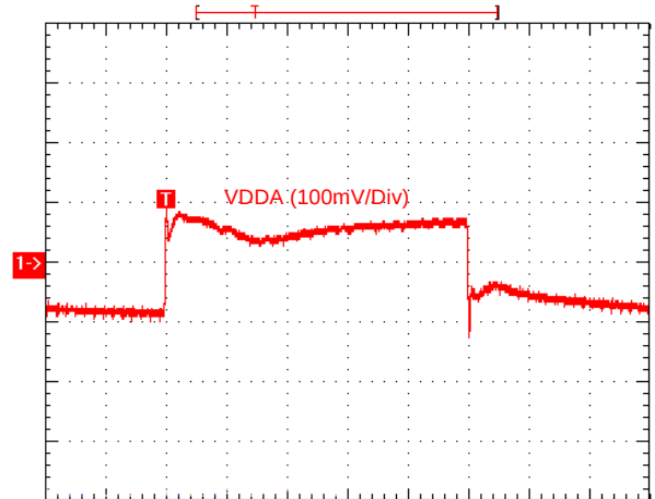
VDDA VR Load Transient
