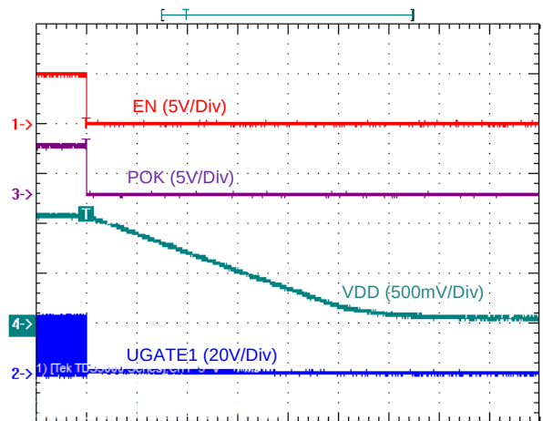
VDD VR Power Off from EN
