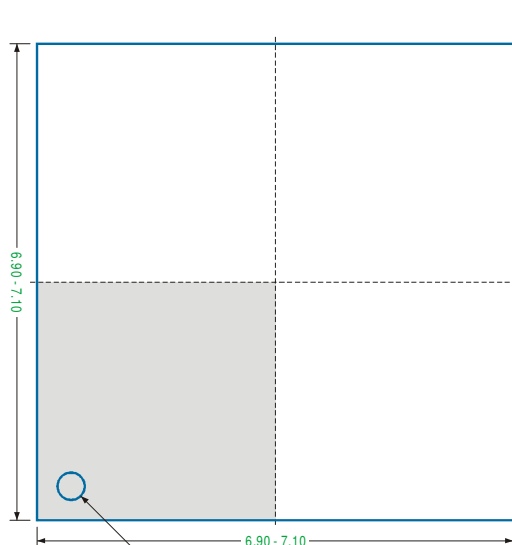
Pin 1 mark
