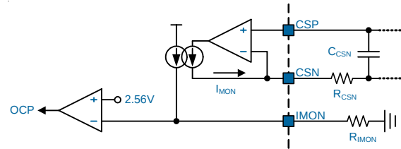
Figure 7. Total Output OCP
