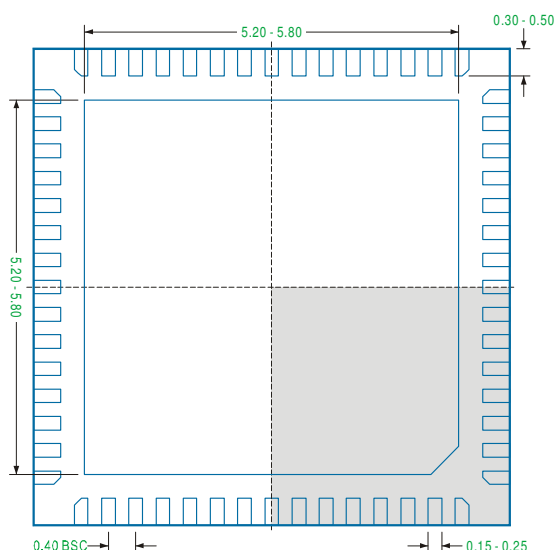
Bottom View - Exposed Pad
