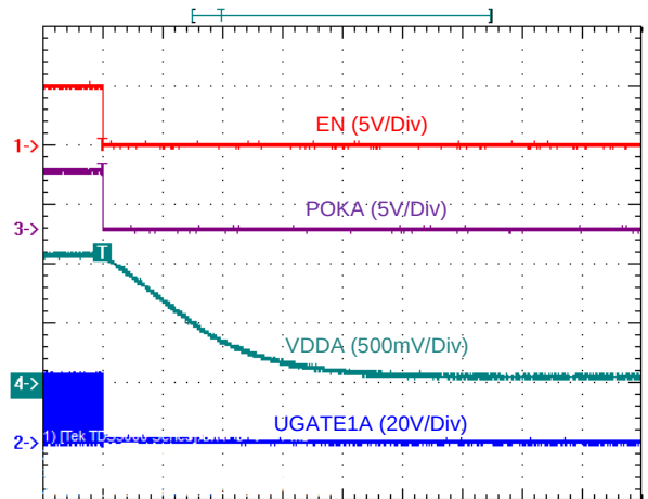
VDDA VR Power Off from EN
