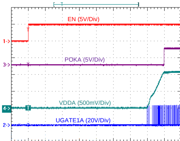
VDDA VR Power On from EN
