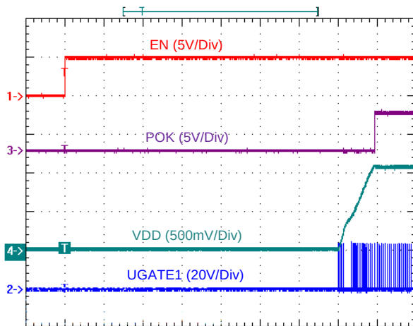
VDD VR Power On from EN
