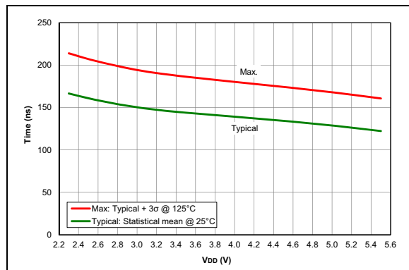
FIGURE 36-87: Comparator Response Time Falling edge, PIC16F18324/18344 Only
