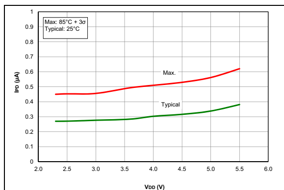
FIGURE 36-25: IPD BASE, 11, PIC16F18324/18344 Only
