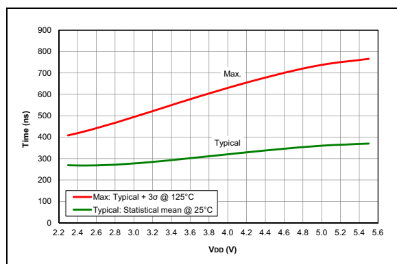
FIGURE 36-89: Comparator Response Time Rising edge, PIC16F18324/18344 Only
