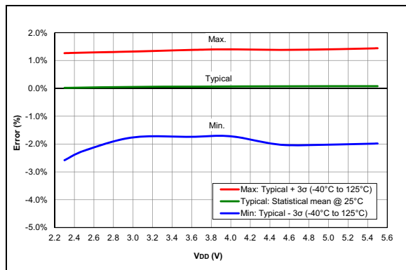
FIGURE 36-27: HFINTOSC Typical Frequency Error, PIC16F18324/18344 Only
