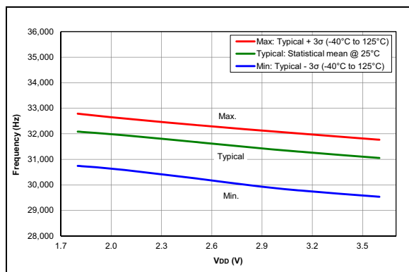
FIGURE 36-29: LFINTOSC Frequency, PIC16LF18324/18344 Only
