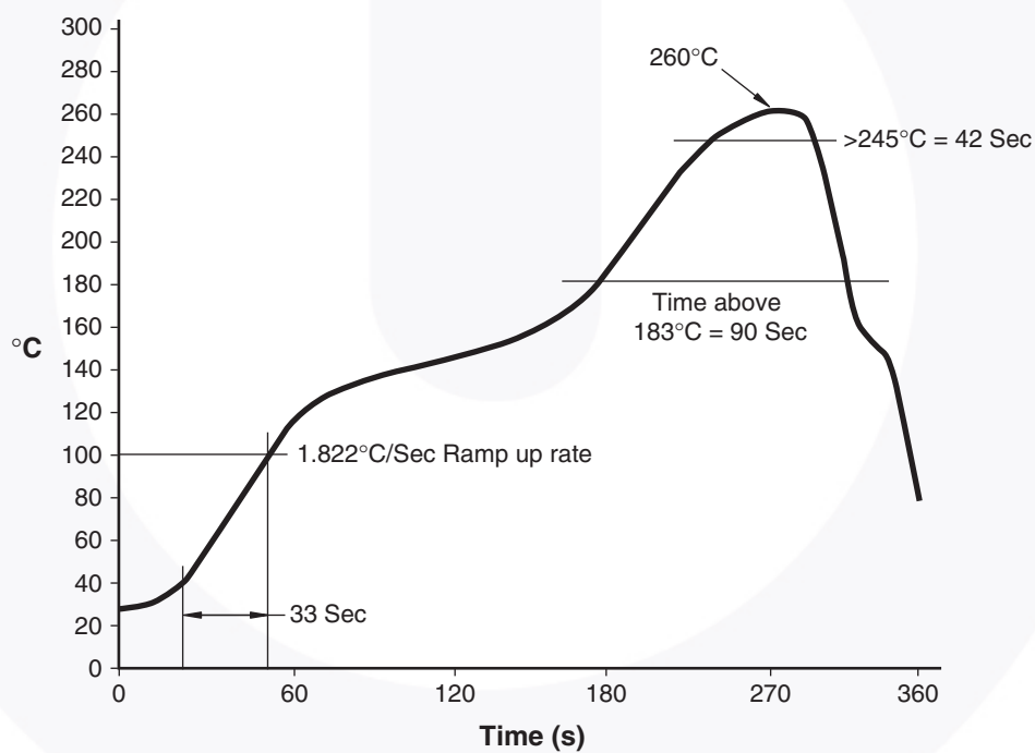
Figure 10. Reflow Profile
