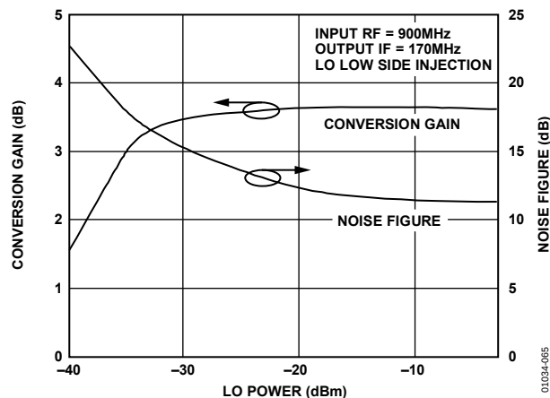
Figure 65. Gain and Noise Figure vs. LO Input Power
