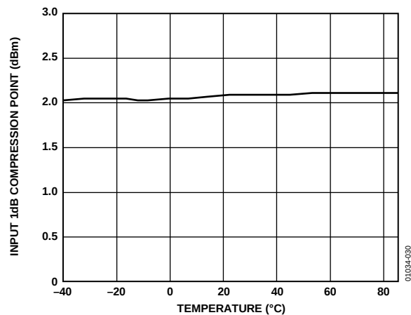
Figure 30. Input 1 dB Compression Point Performance Over Temperature; f_{IN} = 2400 \text{ MHz} , f_{OUT} = 170 \text{ MHz}
