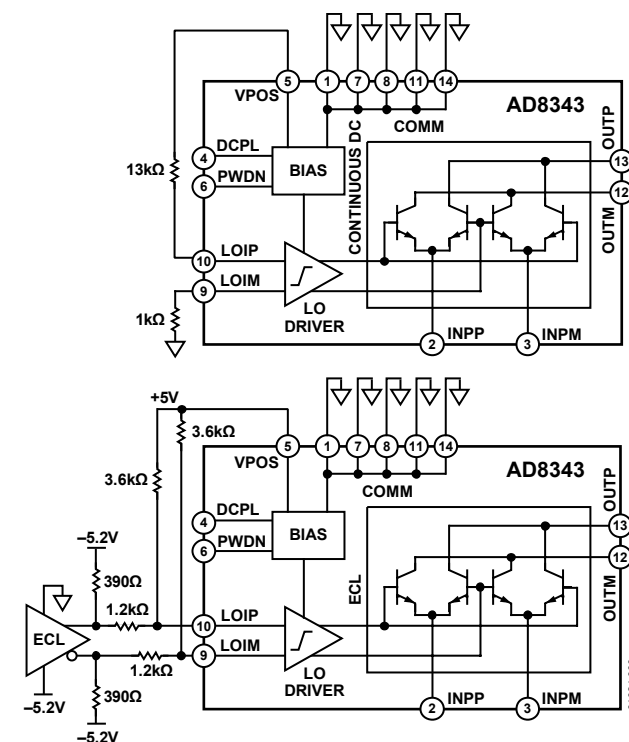
Figure 66. DC Interfaces to the LO Port
