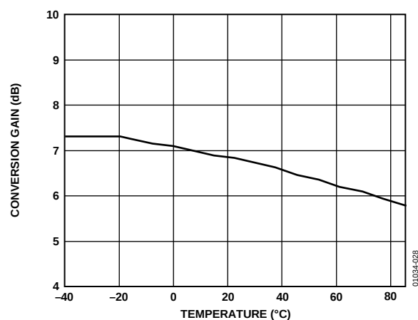
Figure 28. Gain Performance Over Temperature; f_{IN} = 2400 \text{ MHz} , f_{OUT} = 170 \text{ MHz}
