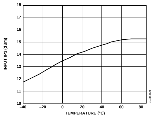
Figure 29. Input IP3 Performance Over Temperature; f_{IN} = 2400 \text{ MHz} , f_{OUT} = 170 \text{ MHz}
