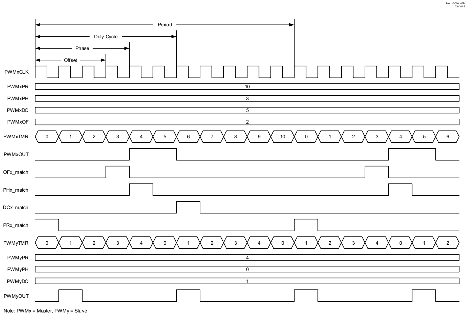
FIGURE 22-8: INDEPENDENT RUN MODE TIMING DIAGRAM
