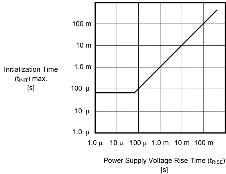
Figure 27 Initialization Time of S-24C512C
