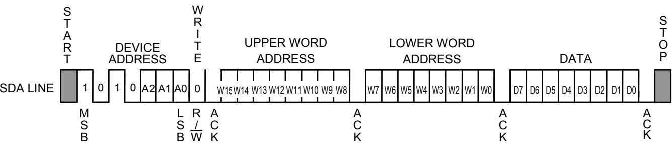
Figure 12 Byte Write
