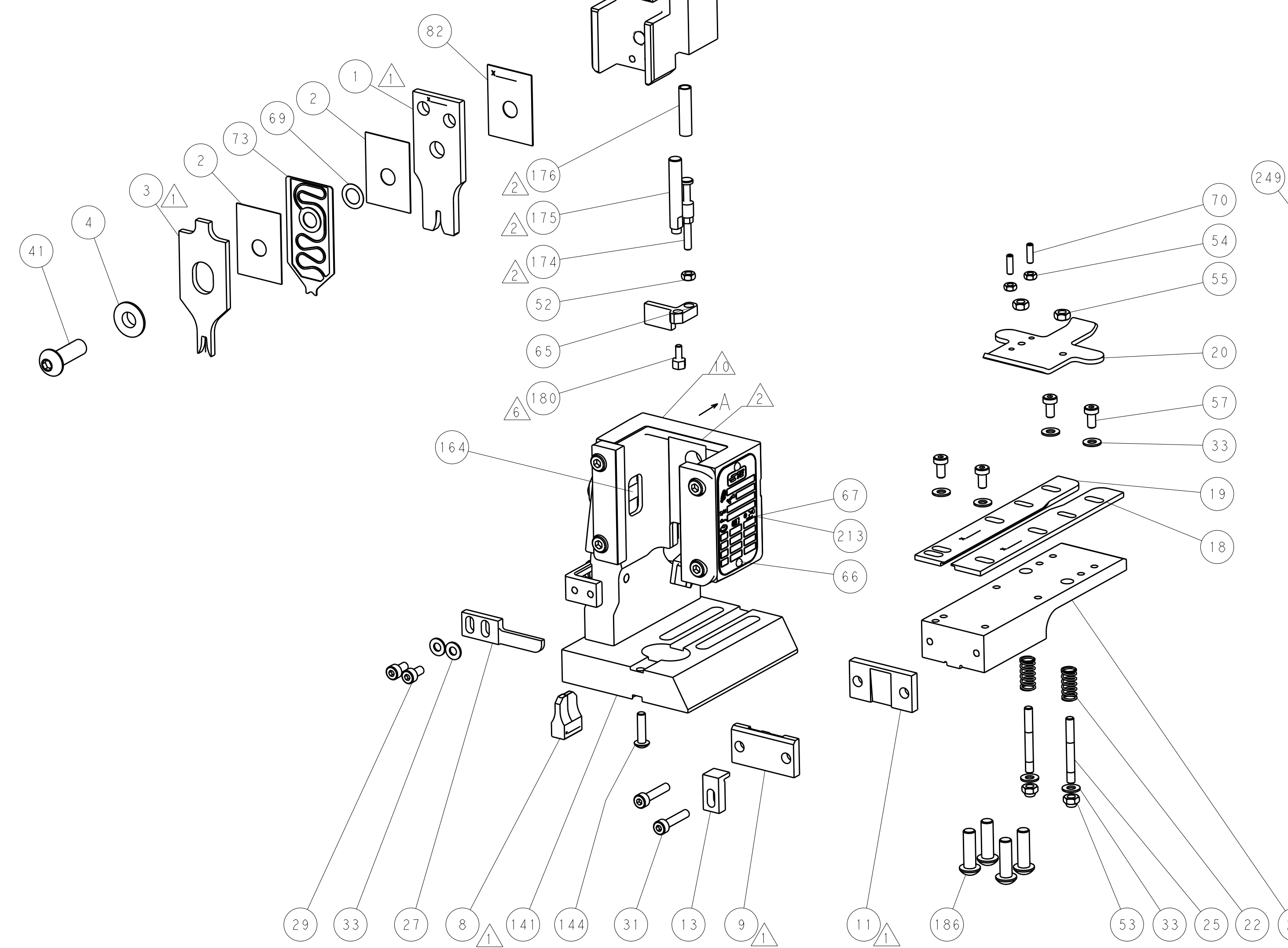
SERVO LATCH PLATE
