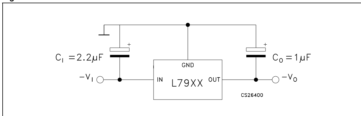
Figure 3. Test circuit
