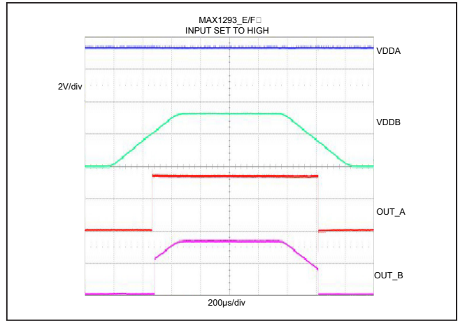
Figure 6. Undervoltage Lockout Behavior (MAX1293_B/C Low)
