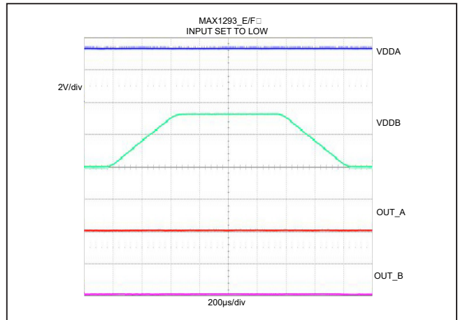
Figure 8. Undervoltage Lockout Behavior (MAX1293_E/F Low)
