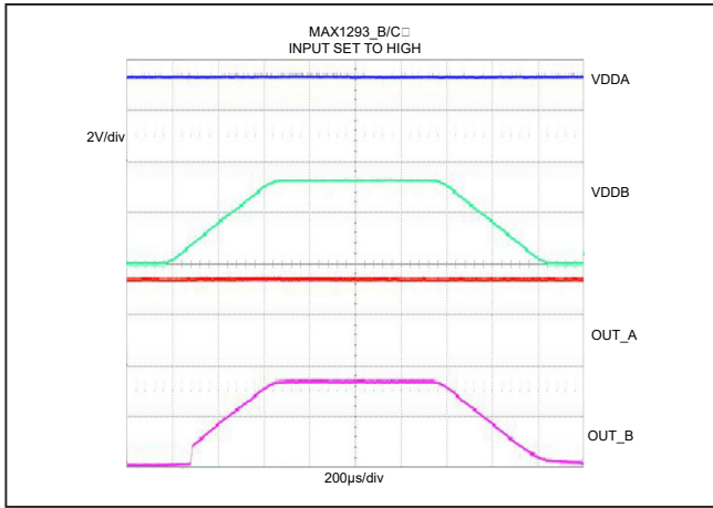
Figure 5. Undervoltage Lockout Behavior (MAX1293_B/C High)
