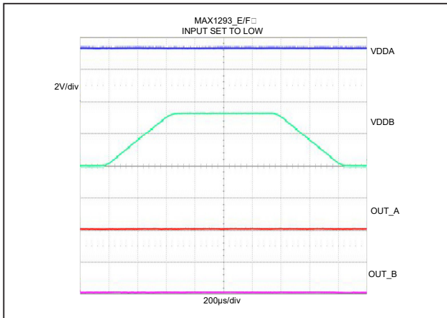
Figure 7. Undervoltage Lockout Behavior (MAX1293_E/F High)
