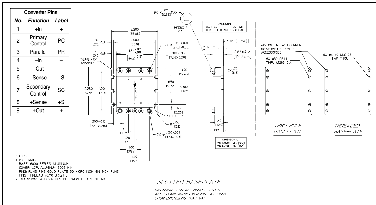
Figure 13 — Module outline
