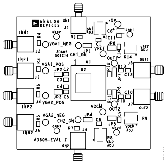
Figure 45. AD605-EVALZ Assembly
