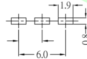
P.C.B MOUNTING PATTERN
