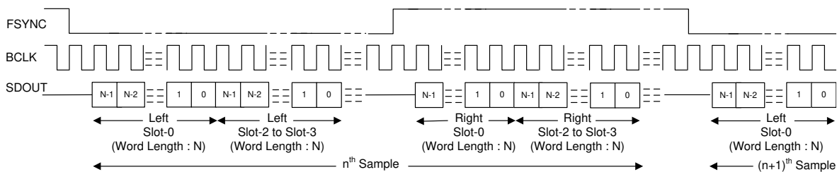
Figure 8-9. I²S Protocol Timing (TX_OFFSET = 0 and BCLK_POL = 1)
