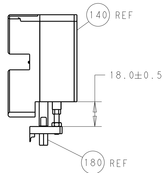
HOLDDOWN SET-UP
