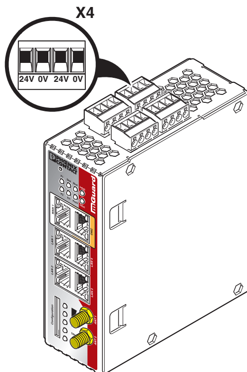
Figure 4 Power supply
