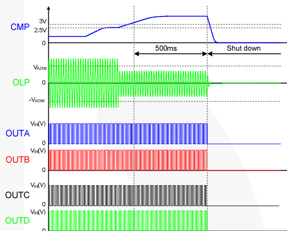
Figure 46. CMP-High Protection in Normal Mode
