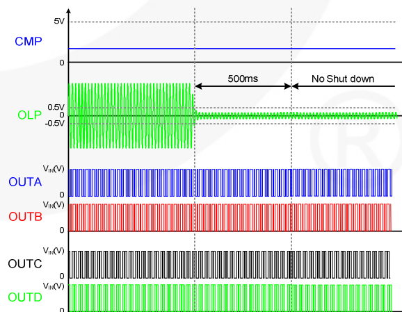
Figure 43. Open-Lamp Protection in DCR Mode
