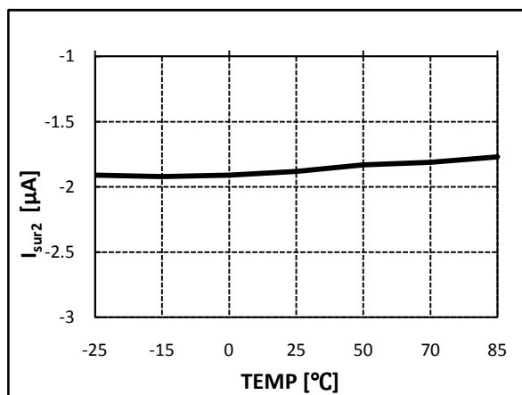
Figure 14. Error Amplifier Source Current 2 vs. Temperature
