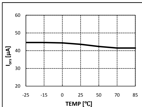
Figure 18. OLR Error Amplifier Sink Current vs. Temperature
