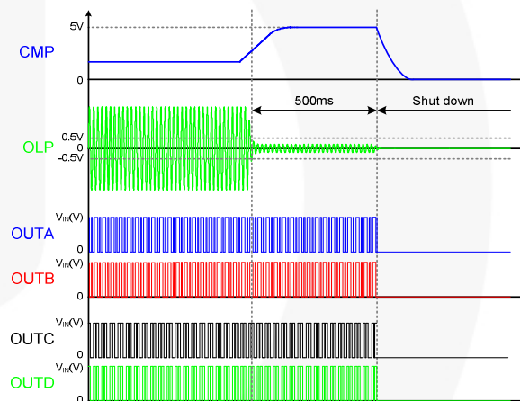
Figure 42. Open-Lamp Protection in Normal Mode
