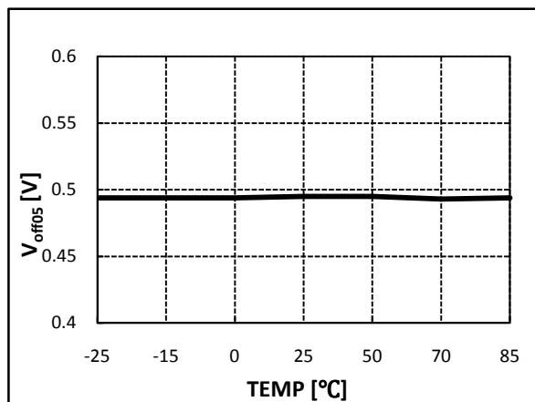
Figure 12. Error Amplifier Offset 05 vs. Temperature
