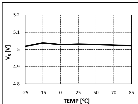
Figure 8. 5V Regulation Voltage vs. Temperature
