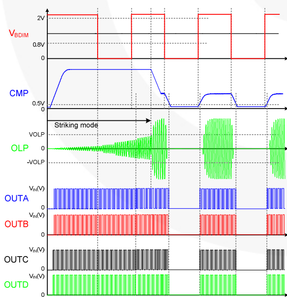
Figure 33. Burst-Dimming During Striking Mode
