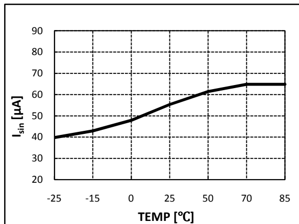
Figure 16. Error Amplifier Sink Current vs. Temperature
