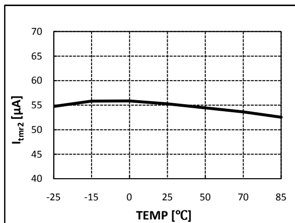
Figure 28. TIMER Current 2 vs. Temperature
