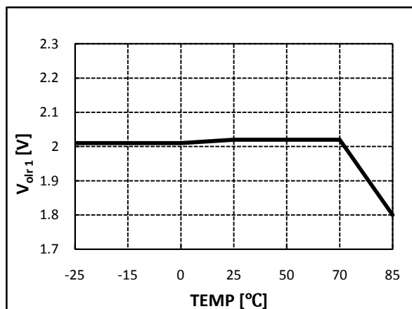
Figure 22. Open-Lamp Regulation Voltage 1 vs. Temperature
