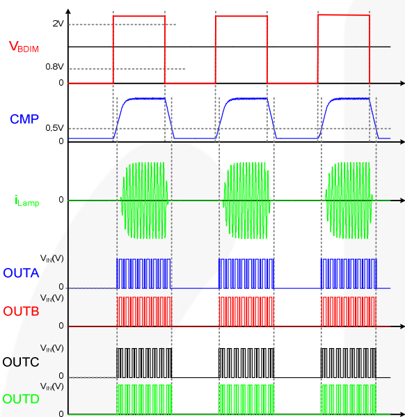
Figure 32. Burst-Dimming Waveforms
