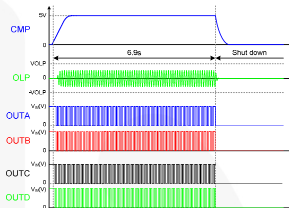
Figure 41. Open-Lamp Protection in Striking Mode
