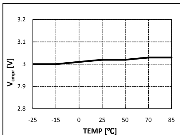
Figure 20. High-CMP Protection Voltage vs. Temperature
