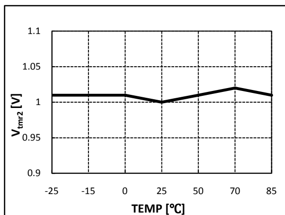
Figure 26. TIMER Threshold Voltage 2 vs. Temperature
