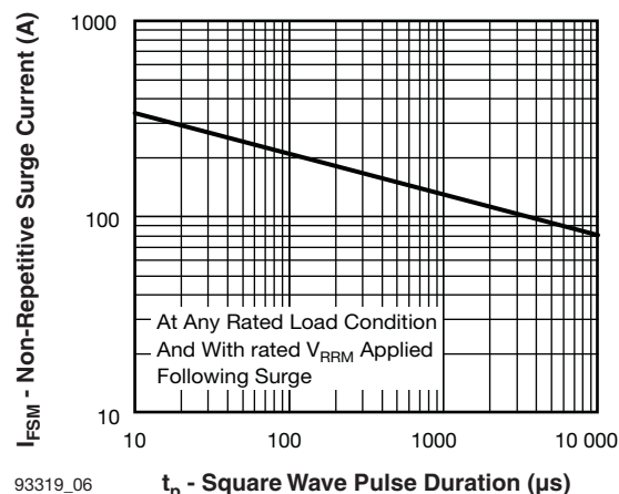
93319_06 t p - Square Wave Pulse Duration (μs) Fig. 6 - Maximum Non-Repetitive Surge Current
