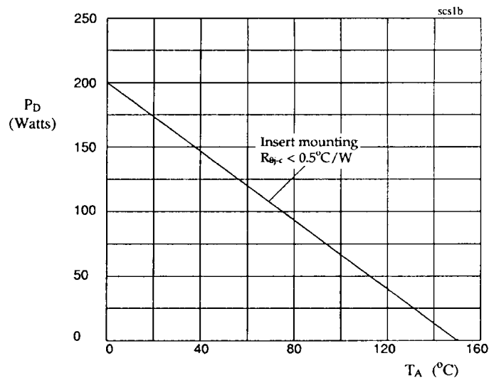
Fig 2. Power dissipation as a function of ambient temperature.
